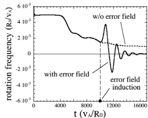
Fig. 1: Nonlinear time evolution of the rotation frequency of magnetic islands. v_A indicates the Alfvén velocity.
