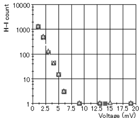
Fig.1 Histogram of the balance voltage signals observed for the LHD helical coils when the NBI was operated, where ■ shows the case including the NBI-induced signals and △ shows the case after removing them.
