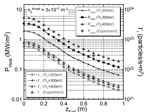
Fig. 3 Axial profile of heat and particle fluxes \blacklozenge : heat flux measurements, \blacktriangle : particle flux measurements, lines: calculation.
