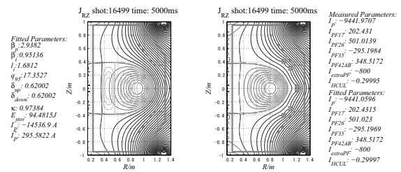
Fig. 2: Magnetic surfaces (red) and current profile (green). In-vessel poloidal field coils are indicated by red squared x markers.
