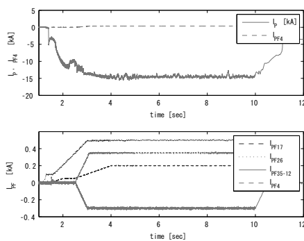
Fig. 1: Time evolution of I_P and I_{PF} .
