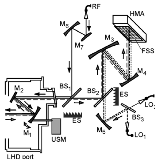
Fig.1 Schematic view of 3-D MIDS in LHD.
