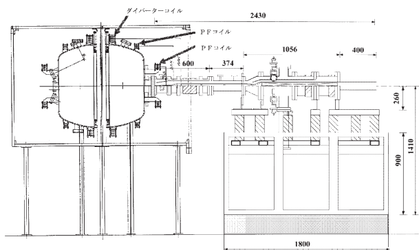
Fig.2 Schematic drawing of the CT injector and the CPD device.
