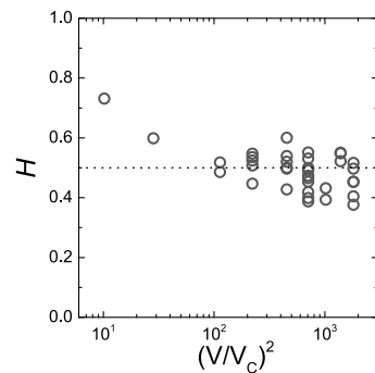
Fig. 3: Experimentally evaluated Hurst number.
