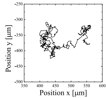
Fig. 1: Orbit of tracer particle in an EHC turbulence.
