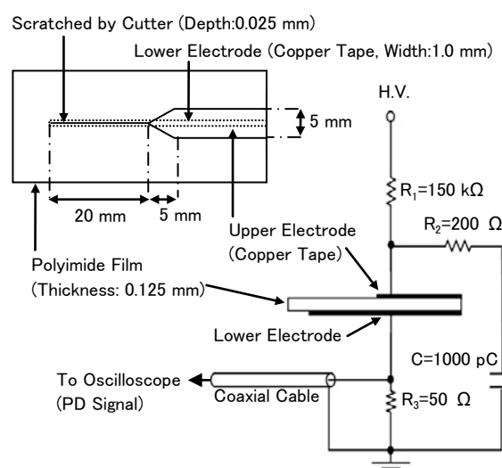
Fig.1 Electrode configuration and experimental setup.
