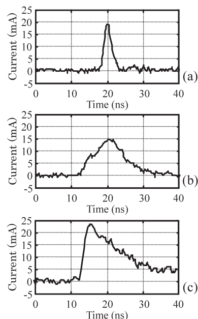
Fig.2 Typical PD current waveform
