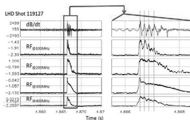
Fig.3 : dB/dt and RF radiations during the EIC. Right figures are expansion of the burst.
