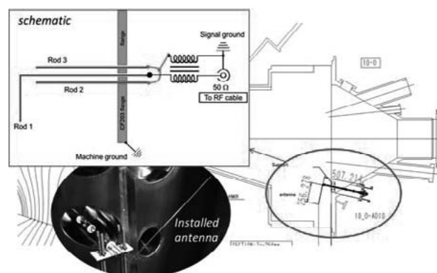
Fig. 1: Dipole antenna installed inside the vessel at the 10-O port.
