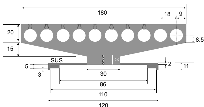
Fig. 1 Fig.1 Detail design of heat transfer block
