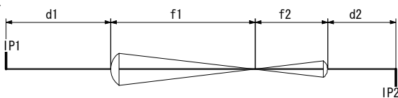
Fig. 1. A schematic diagram of the Keplerian image relay telescope. Focal lengths of convex lenses are f1 and f2 . IP1 and IP2 are image point of this optical system. d1 and d2 are the distance between lens and image.
