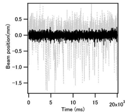
Fig. 3. A beam position of TS beam line at the 40 m from the laser output. Gray line is without image relay. Black line is with image relay.
