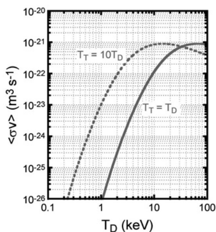
Fig. 1 Enhancement of fusion reactivity by having high-energy tritons with 10 times the temperature of bulk deuterons. The horizontal axis is taken as the bulk deuteron temperature.
