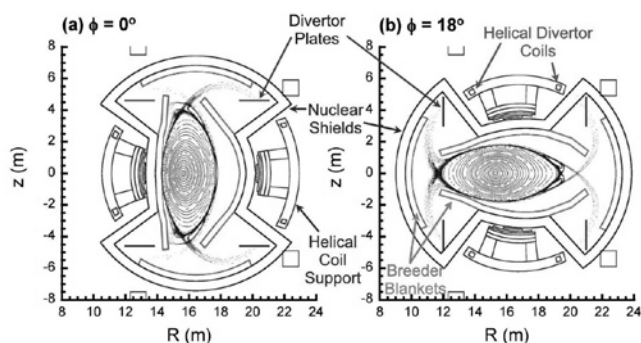
Fig. 1 Vacuum magnetic surfaces and divertor legs of FFHR-2m2 at two toroidal cross-sections including the field changes provided by the helical divertor coils.
