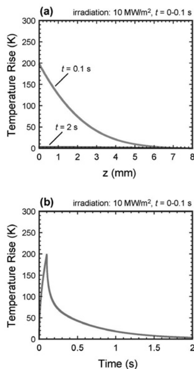
Fig. 2 (a) Temperature distribution in a tungsten slab at times of t = 0.1 and 2 s with a heat flux of 10 MW/m 2 applied to the z = 0 mm surface during t = 0-0.1 s. (b) Temperature rise as a function of time at z = 0 mm.
