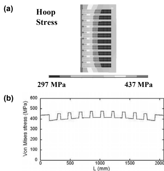
Fig. 2 (a) Distribution of hoop stress in a solenoid coil model of the FFHR helical coil by considering the radial electromagnetic force. (b) The Von Mises equivalent stress along the innermost layer of the coil case.
