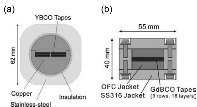
Fig. 1. Cross-sectional images of (a) the 100kA-class HTS conductor designed for the FFHR-d1 helical coils and of (b) the prototype conductor sample.
