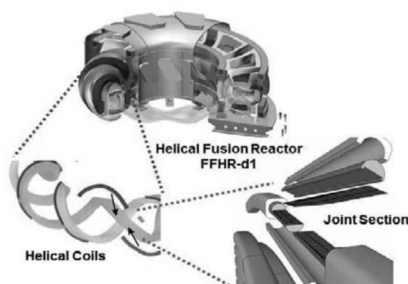
Fig. 2. Schematic illustration of “joint-winding” to be applied to the FFHR-d1 helical coils.
