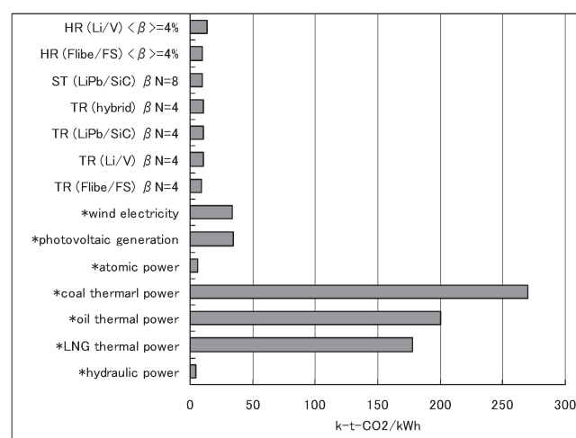
Fig.2. CO 2 emission amount per electric energy output 3) *) referred from Y. Uchiyama Socio-economic Research Center, Y94009, (1995)
