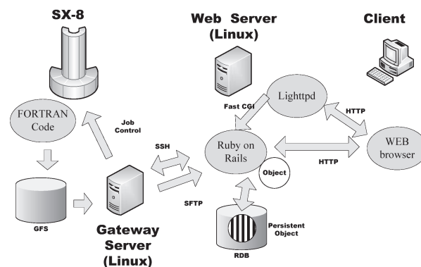
Fig. 2. System Layout of LHD Data Analysis Interface
