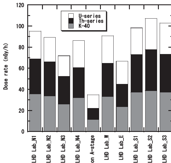
Fig. 2 Dose rate in LHD Lab.
