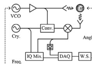
Fig. 1 Block diagram of microwave scattering CT system.
