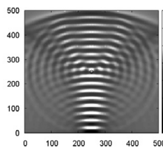
Fig. 2. Scattering pattern calculated by FDTD method.
