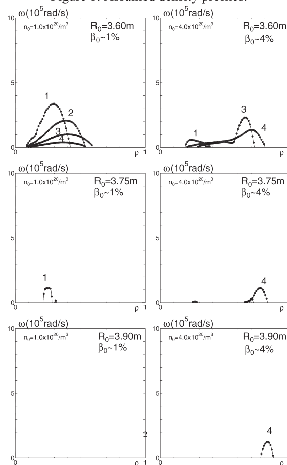
Figure 2: Ballooning growth rate as a function of \rho in R_0=3.60\text{m} (top), R_0=3.75\text{m} (mid) and R_0=3.90\text{m} (bottom) configurations of LHD. Left (right) column corresponds to the 1% (4%) central beta cases.
