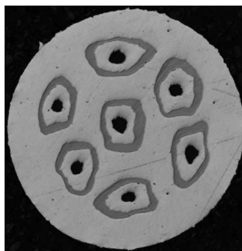
Fig.3 Typical optical microscopic photograph of the high mechanical strength Bi-2212 multifilamentary round wire using metal Ni sheath material (Sample C).
