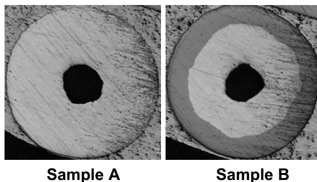
Fig.2 Typical optical microscopic photographs of the high mechanical strength Bi-2212 mono-cored round wire using metal Ni sheath material (Sample A and B).
