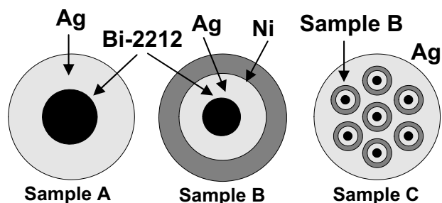
Fig. 1 Typical cross-sectional configuration of high mechanical strength Bi-2212 round wire using metal Ni sheath material.
