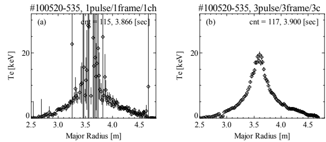
Fig. 2. (a) T_e profile without simultaneous laser firing and data accumulation methods, (b) simultaneous laser firing and all data accumulation methods were applied.
