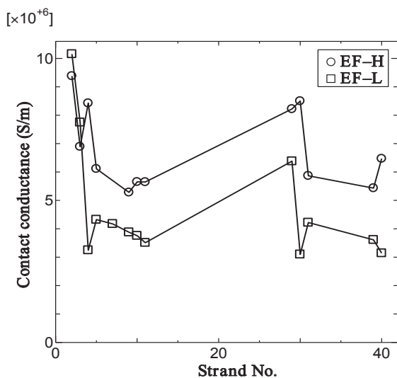
Fig. 1. Measured contact conductance for various combinations of strands. The numbers on the horizontal axis are proportional to the distance between a pair of strands.
