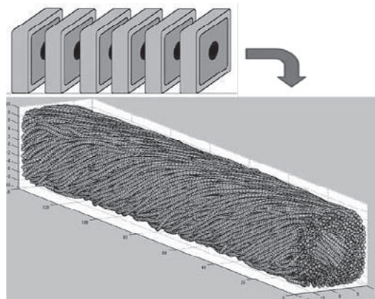
Fig. 2. Experimentally obtained strand traces of EF-L conductor of JT-60SA.
