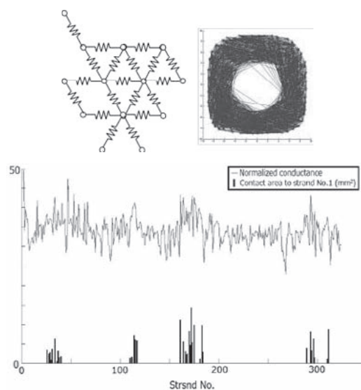
Fig. 3. Contact conductance vs. the number of strand (i.e. distance between strands). The bar graph indicates the calculated area of the contact crossover.
