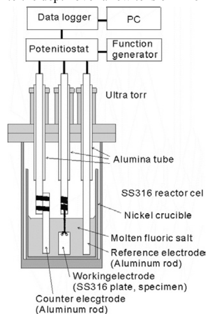
Fig. 1. Experiment setup for electrochemical measurement and treatment.
