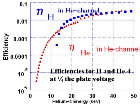
FIG. 1. (Color online) Efficiencies for He-4 and scattered hydrogen at the plate voltage of 1/4 times of hydrogen. Even if the plate voltage is adjusted to the He channel, the scattered hydrogen is still observed.
