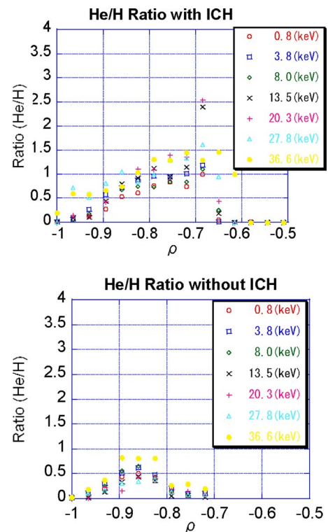
FIG. 4. (Color online) Helium profiles with/without HHFW heating. The higher flux of He can be observed during the HHFW heating.
