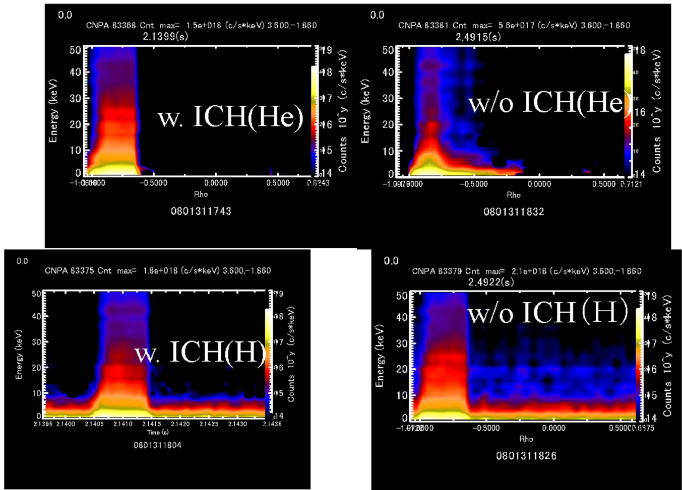
FIG. 3. (Color online) Four PCX signals set on He channel and H channel with/without HHFW heating. To confirm helium acceleration, we compare four different PCX signals.
