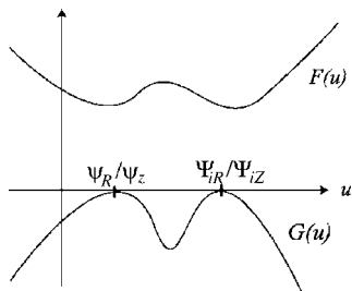
FIG. 1. Sketch of F(u) and G(u) .
