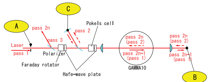
FIG. 3. Schematic diagram of the multi-pass system.
