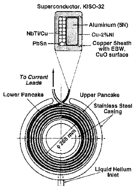
Fig. 2 Schematic drawing of a double pancake coil, HELIUT. The internal structure of the superconductor is also shown.
