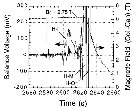
Fig. 1 Waveforms of the balance voltage signals measured for the three blocks of the helical coils, during a quench event at a toroidal field of 2.75 T. Magnetic field measured by a Hall probe on the coil-can is also shown.
