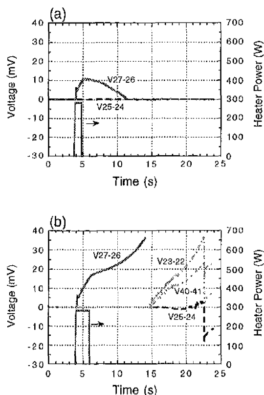
Fig. 5 Voltage signals measured in the R&D helical coil TOKI-HB. (a) A recovery case of a normal zone and (b) a quench case. The voltage tap V27-26 covers the heater installed region at the innermost layer of the winding and V25-24 is the neighboring tap on the same turn. Other taps are on different turns; V23-22 is on the next turn in the same layer and V40-41 on the next layer.
