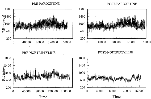
Figure 1. The 24-hour heart period time series for one patient in each drug condition. RR, interbeat interval in milliseconds.
