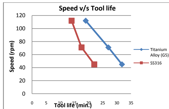
Graph 6: Speed v/s tool life
