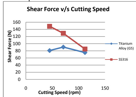
Graph 2: Shear force v/s Cutting speed
