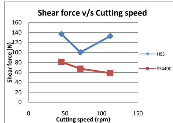
Graph 1: Shear force v/s Cutting speed
