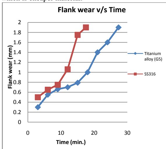
Graph 4: Flank wear v/s Time
