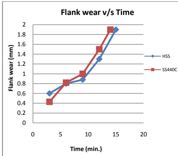
Graph 3: Flank wear v/s Time
