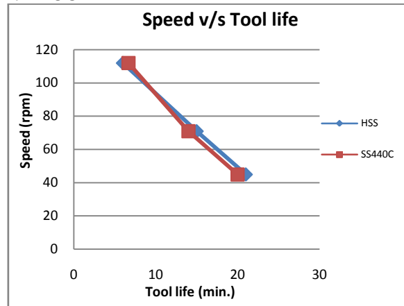
Graph 5: Speed v/s tool life
