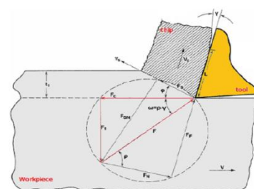
Figure 3: Merchant's Circle Diagram
