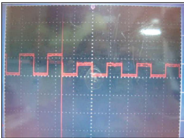
Fig. 10 DAC output when 2kV was given to pin 190
