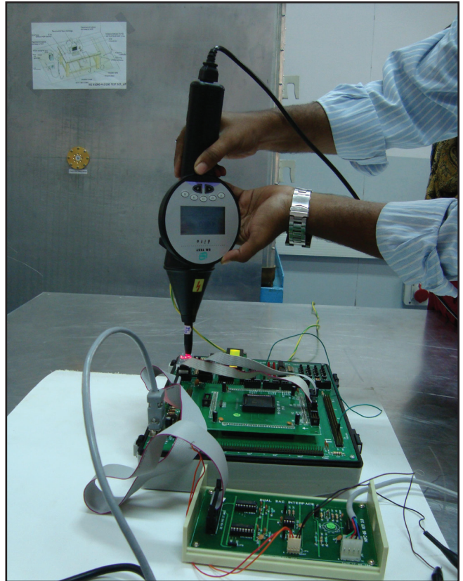
Fig. 4 Air discharge on seven segment display
