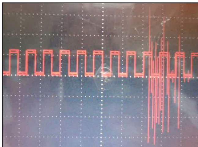
Fig. 8 DAC output for a 8kV discharge
