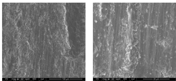
8(d) SEM micrograph of DP810 with 69% martensite volume fraction at 500X and 2000X
