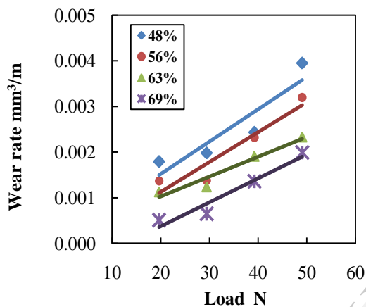
Fig.7. Plot showing variation in wear rate with load for different volume fraction of martensite.
