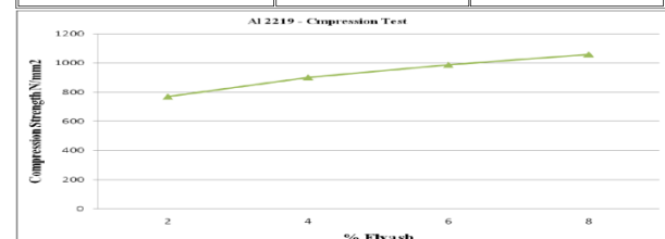
Graph 5.9: Compressive Strength v/s Flyash with 5% E-Glass
