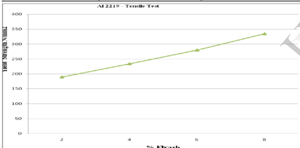
Graph 5.6: Yield Strength v/s Flyash with 5% E-Glass
