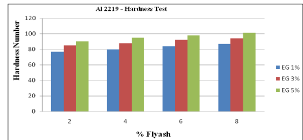
Graph 5.20: Comparative Bar Chart of BHN
