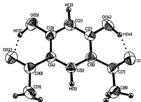
Fig. 1. A perspective view of the molecule with 50% probability thermal ellipsoids.
