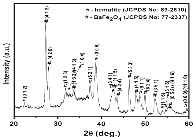
Fig. 1 XRD pattern of microwave-hydrothermally synthesized \text{BaFe}_{12}\text{O}_{19} powder
