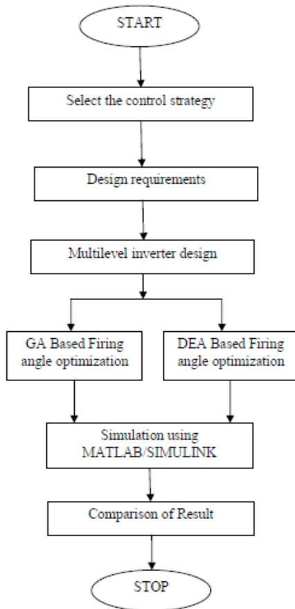
Fig. 3 Flowchart of Methodology
