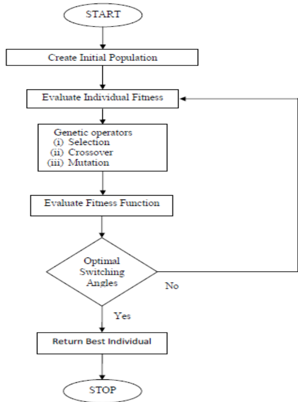
Fig. 4 Flowchart of GA
