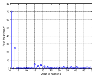
Fig. 9 FFT of Output voltage waveform result of DEA of MI=0.7
