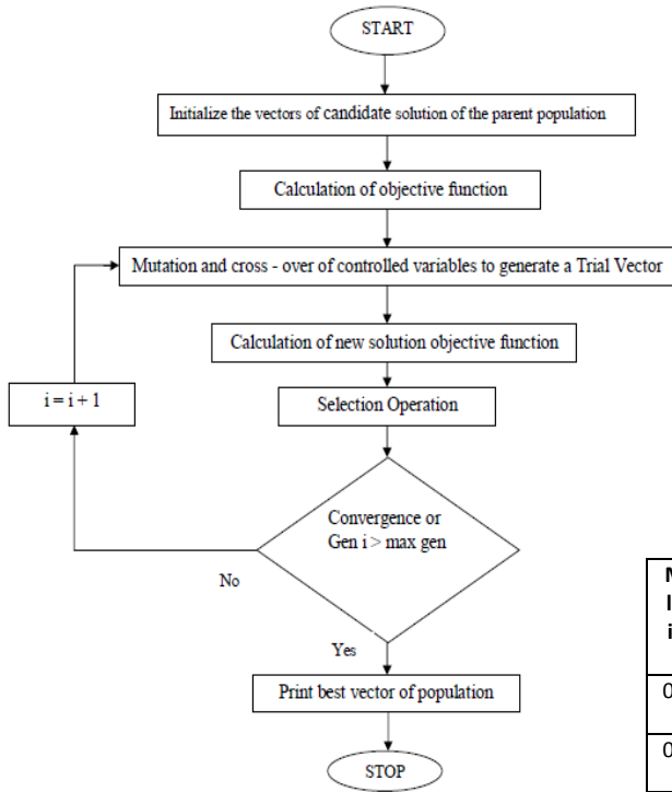
Fig. 5 Flowchart of DEA
