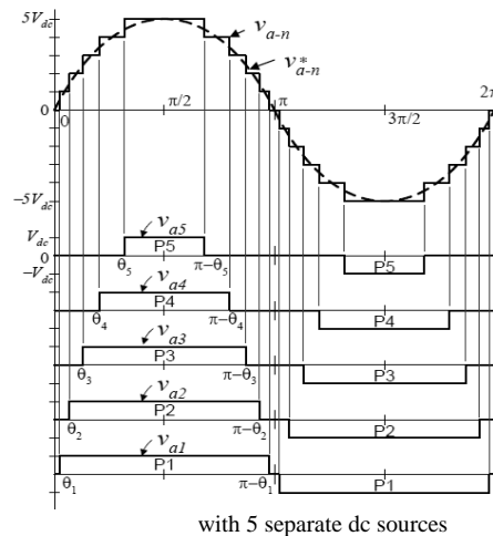
Fig.2 Output phase voltage waveform of an 11-level cascade inverter
