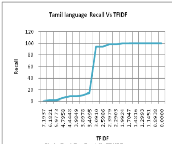
Fig 5 : Tamil Text Recall Vs TF*IDF
