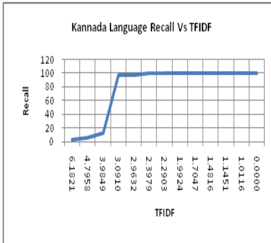
Fig. 4 : Kannada text Recall Vs TF*IDF
