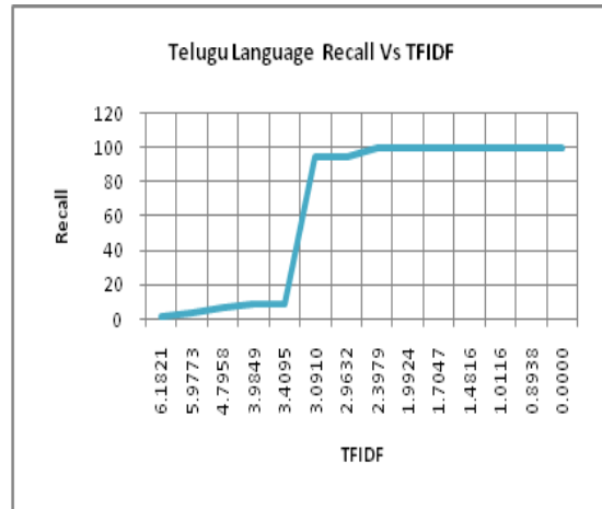
Fig 6 : Telugu Text Recall Vs TF*IDF
