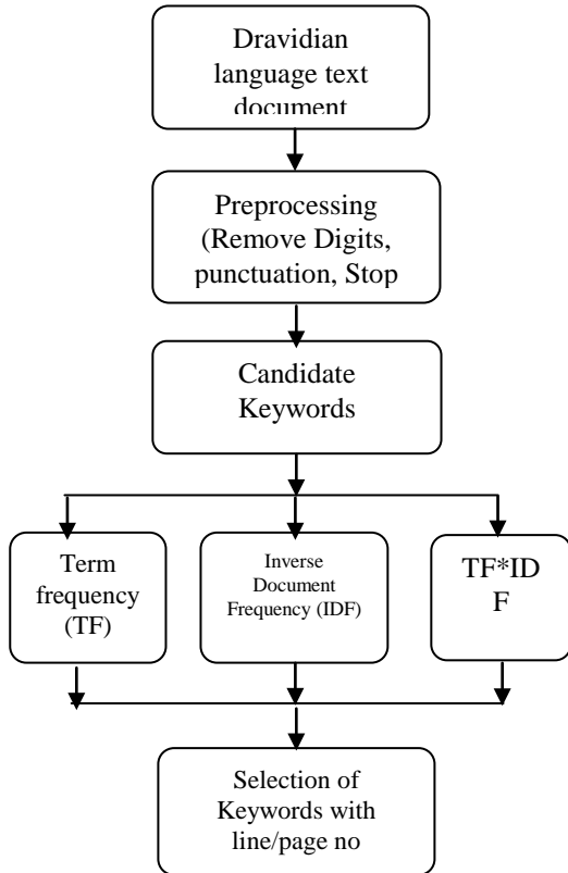
Fig 2. Keywords extraction algorithm
