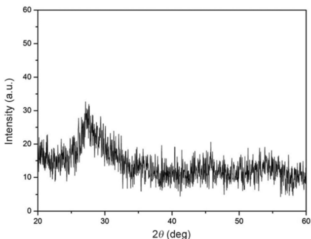
Figure 1. Typical XRD pattern of \text{Eu}_2\text{O}_3-\text{Ag}_2\text{O}-\text{PbO}-\text{B}_2\text{O}_3 glass system.
