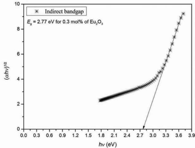
Figure 4. Typical plot of (\alpha h\nu)^{1/2} vs. h\nu for indirect bandgap measurement in x\text{Eu}_2\text{O}_3-(1-x)\text{Ag}_2\text{O}-29\text{PbO}-70\text{B}_2\text{O}_3 glass with x = 0.3 mol%.
