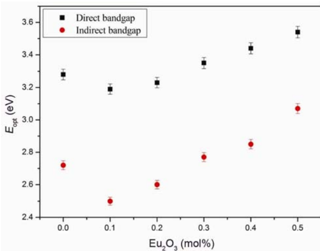
Figure 5. Variation of direct and indirect bandgap as a function of \text{Eu}_2\text{O}_3 mol%.
