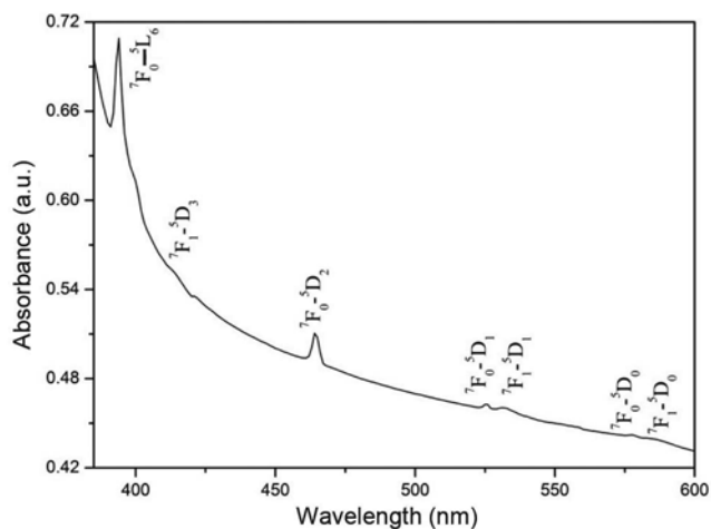
Figure 2. Typical optical absorption spectra of (1-x)\text{Ag}_2\text{O}-29\text{PbO}-70\text{B}_2\text{O}_3 with x = 0.5 \text{ mol\%} of \text{Eu}_2\text{O}_3 .
