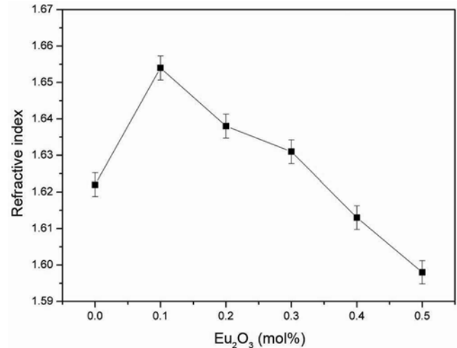
Figure 6. Variation of refractive index as a function of \text{Eu}_2\text{O}_3 mol%.
