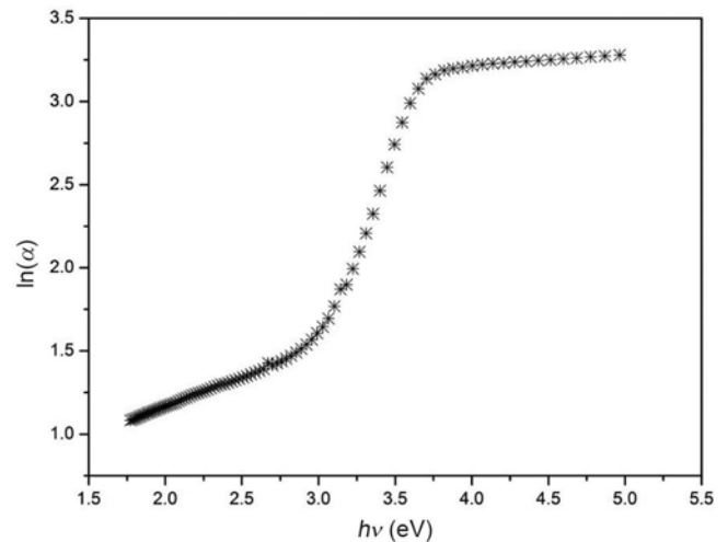
Figure 7. Typical plot of \ln(\alpha) vs. h\nu for Urbach energy measurements in \text{Eu}_2\text{O}_3-\text{Ag}_2\text{O}-\text{PbO}-\text{B}_2\text{O}_3 glass system.
