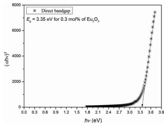
Figure 3. Typical plot of (\alpha h\nu)^2 vs. h\nu for direct bandgap measurement in x\text{Eu}_2\text{O}_3-(1-x)\text{Ag}_2\text{O}-29\text{PbO}-70\text{B}_2\text{O}_3 glass with x = 0.3 \text{ mol\%} .
