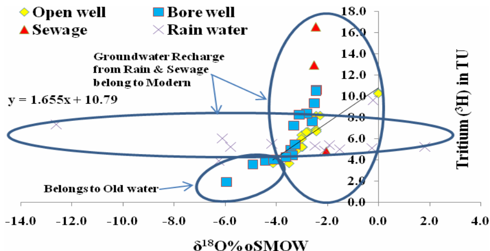
Figure 6. Plot of ^3\text{H} vs. \delta^{18}\text{O} ‰ SMOW of sewage, rain water, open and bore well samples.
