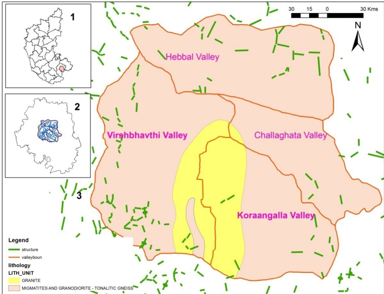
Figure 2. Geological background of Challaghatta with surrounding valleys.
