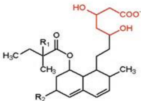
Figure 1. Structure of Lovastatin
