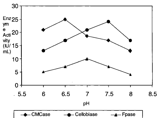
Figure 1. Effect of PH on enzyme production by Clostridium papyrosolvans CFR-703.
