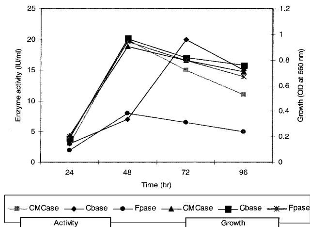
Figure 3. Kinetics of scaled-up enzyme production by Clostridium papyrosolvens CFR-703.
