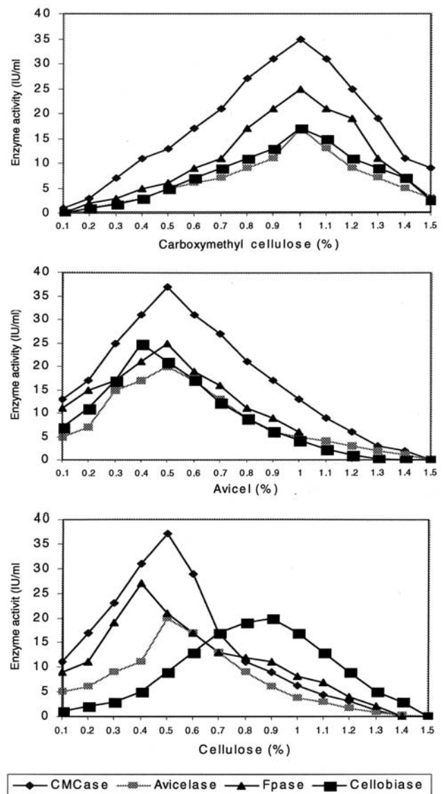
Figure 2. Effect of various concentrations of carboxymethylcellulose, avicel and cellulose on enzyme production by Clostridium papyrosolvans CFR-703.
