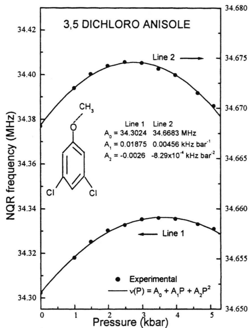
Fig. 3. Variation of ^{35}\text{Cl} NQR frequency with pressure in 3,5-dichloroanisole.
