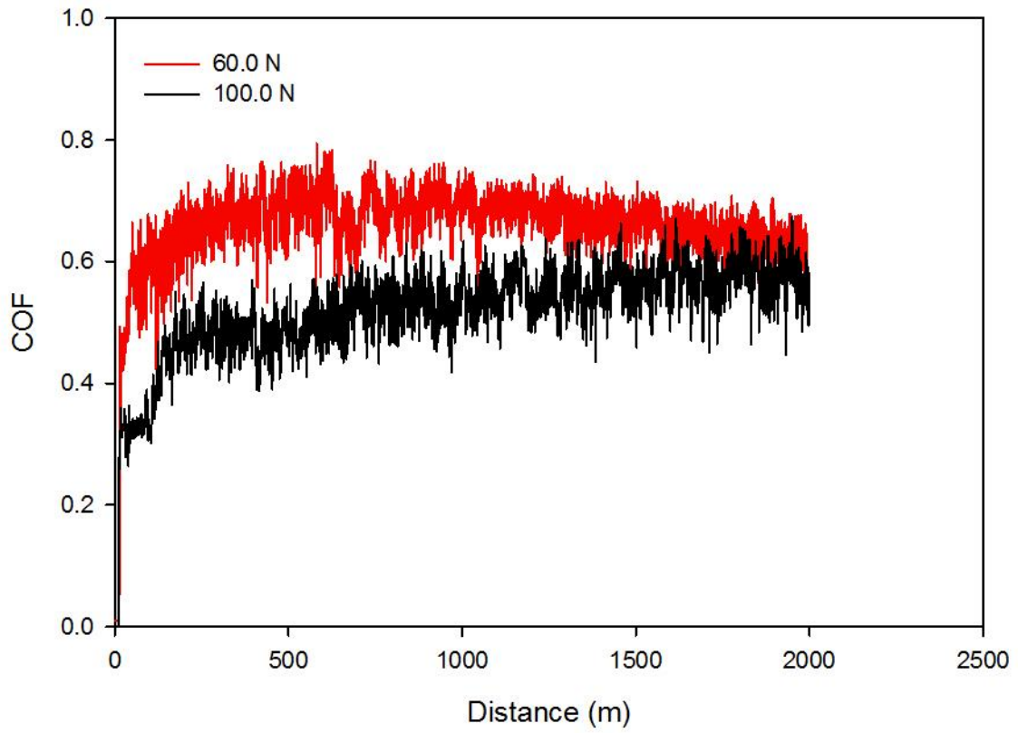
Figure 4.50. COF plots for AM60-9% (Al_2O_3)_f composite tested at 0.1 m/s
