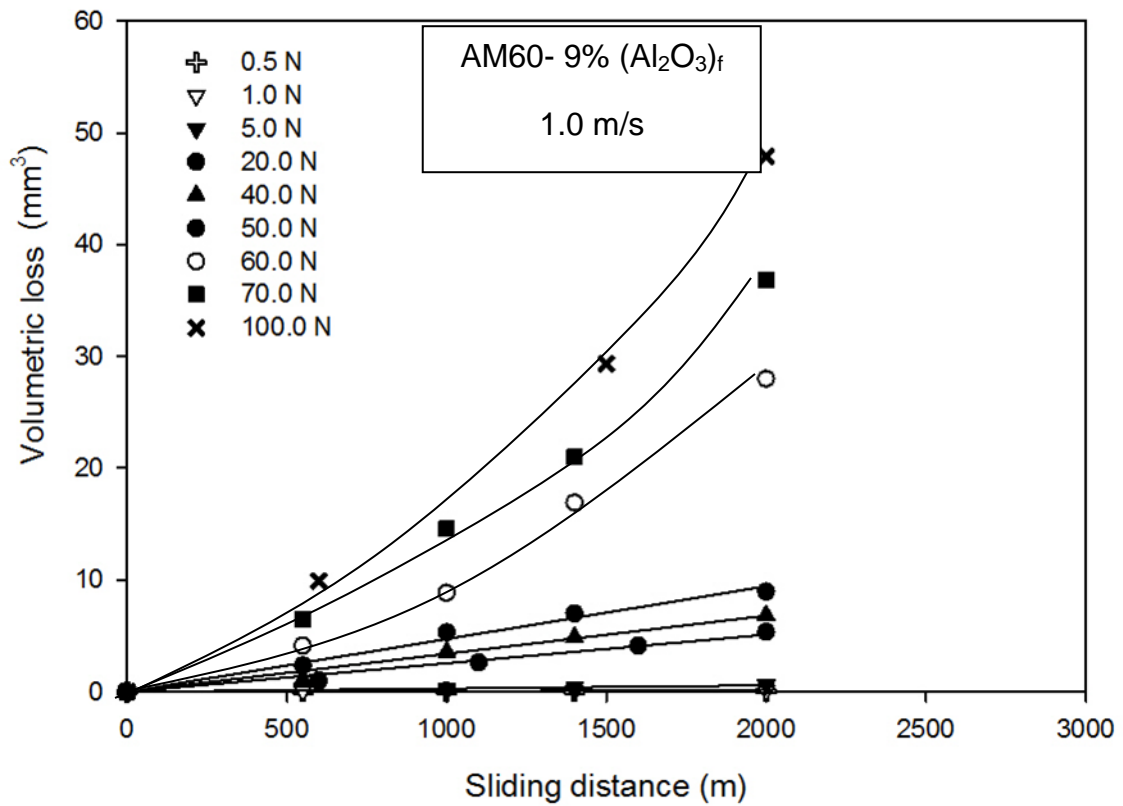
Figure 4.11. Volumetric loss vs. sliding distance plots for various tested loads at 1.0 m/s for AM60- 9% (Al 2 O 3 ) f composite.
