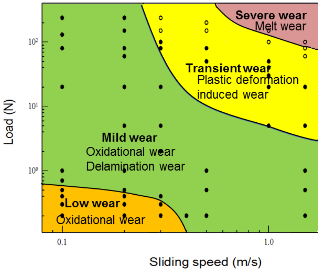
Figure 4.40. Wear map for AM60 alloy
