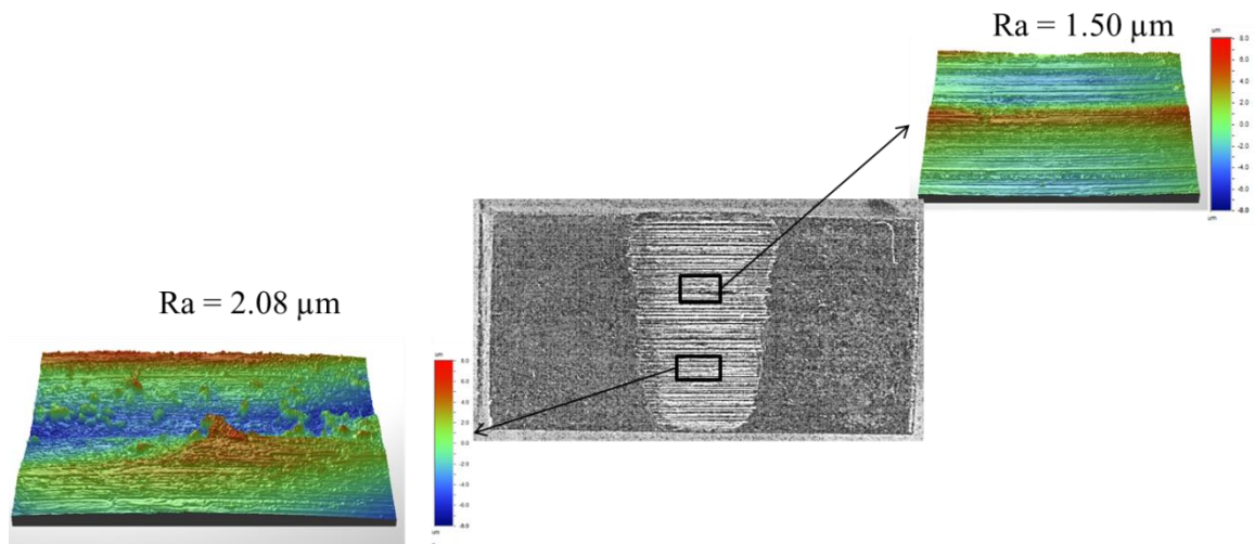
Figure 5.7. 3D profiles showing high roughness all over the worn surface mapped on stereo micrograph for worn surfaces obtained at 60.0 N and 1.5 m/s at 50 m.
