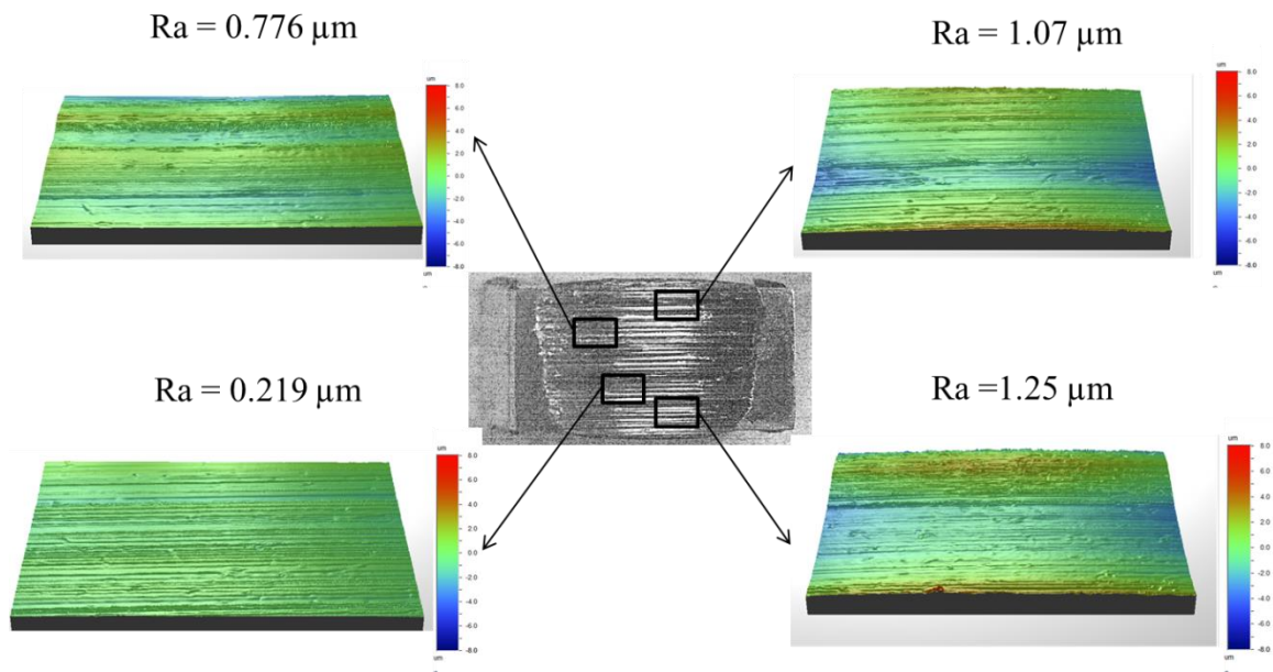
Figure 5.8. 3D profiles showing fluctuating roughness mapped on stereo micrograph for worn surfaces obtained at 60.0 N and 1.5 m/s at 500 m
