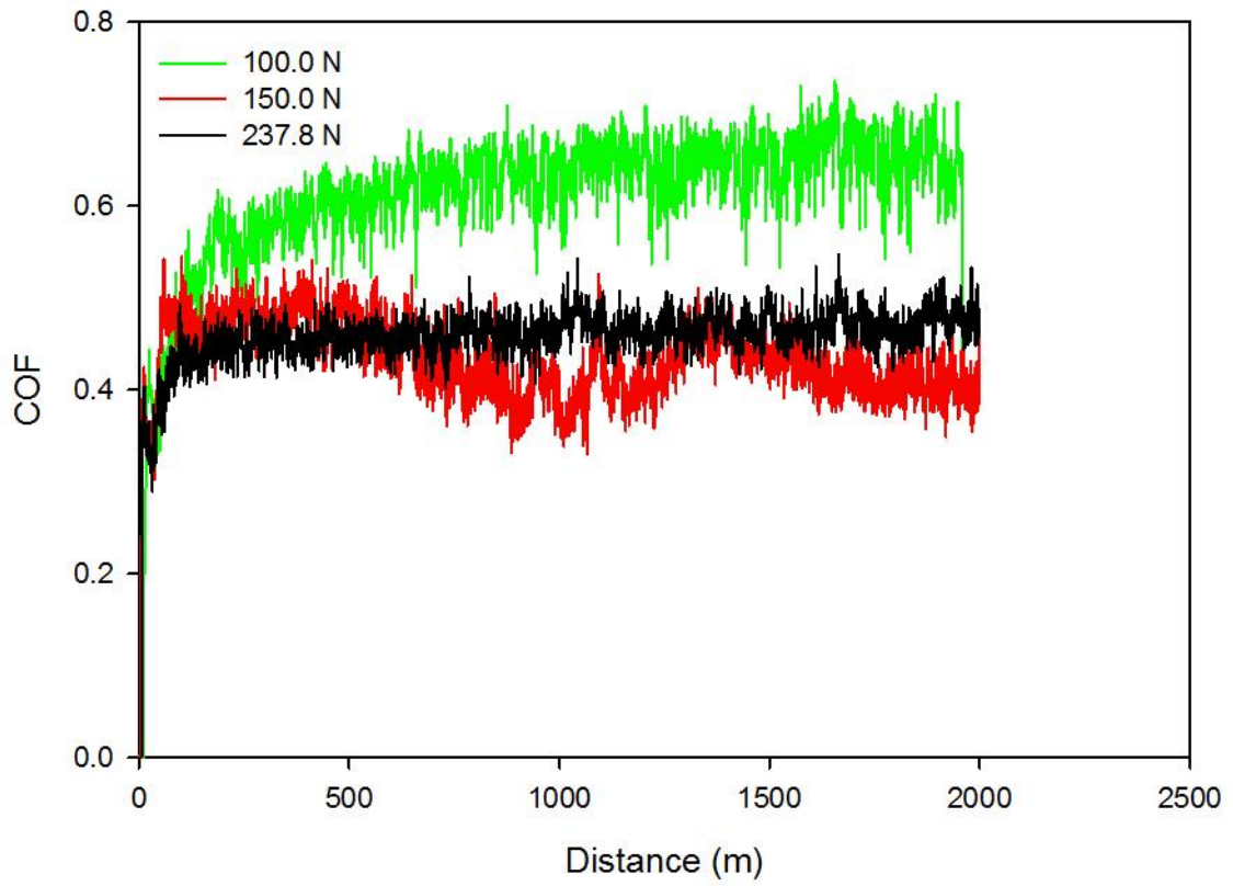
Figure 4.51. COF plots for AM60-9% (Al 2 O 3 ) f composite tested at 0.3 m/s
