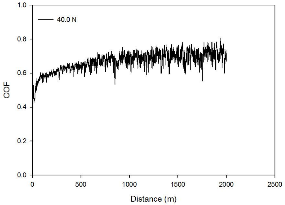
Figure 4.52. COF plots for AM60-9% (Al 2 O 3 ) f composite tested at 1.0 m/s
