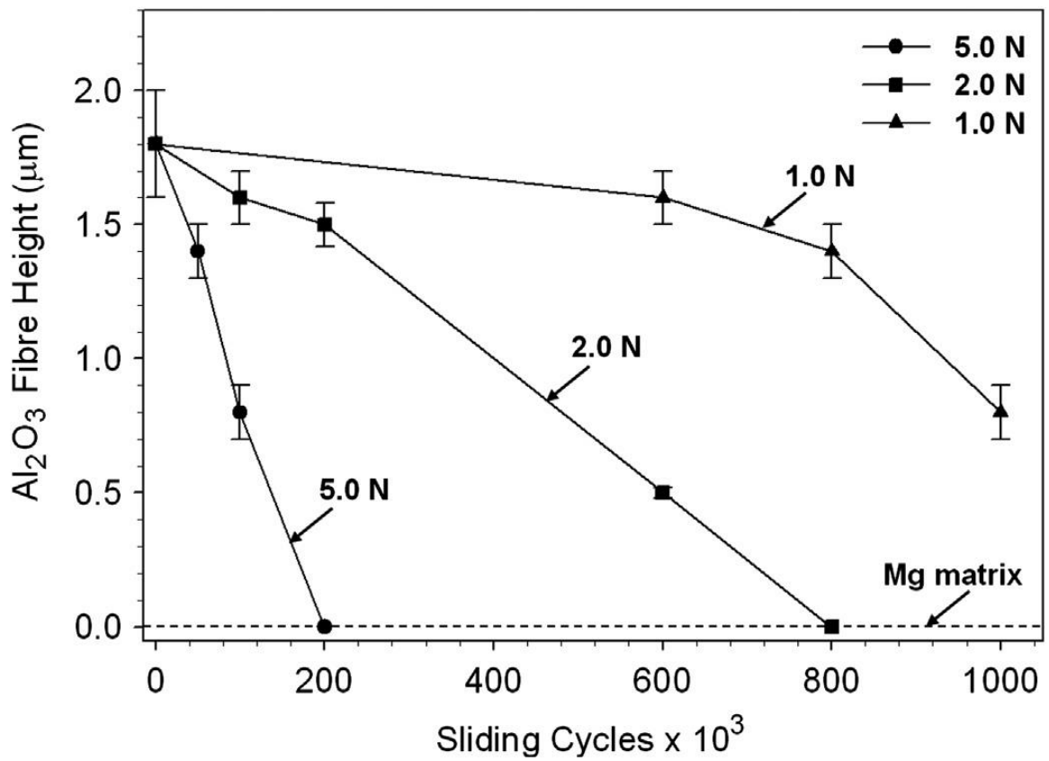
Figure 2.33. Plot of variation of Al 2 O 3 fibre height with sliding cycles at 1.0 N, 2.0 N and 5.0 N for AM60–9% (Al 2 O 3 ) f composite at 25 °C [71].
