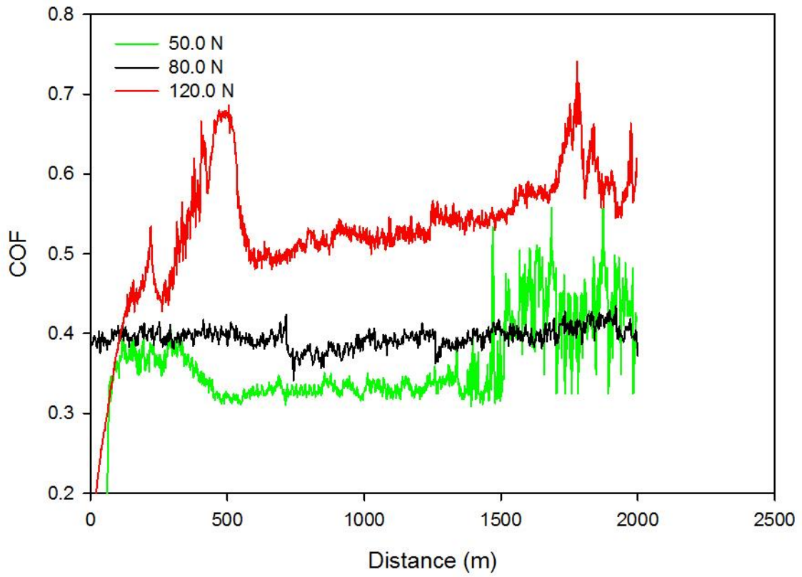
Figure 4.53. COF plots for AM60-9% (Al 2 O 3 ) f composite tested at 1.5 m/s
