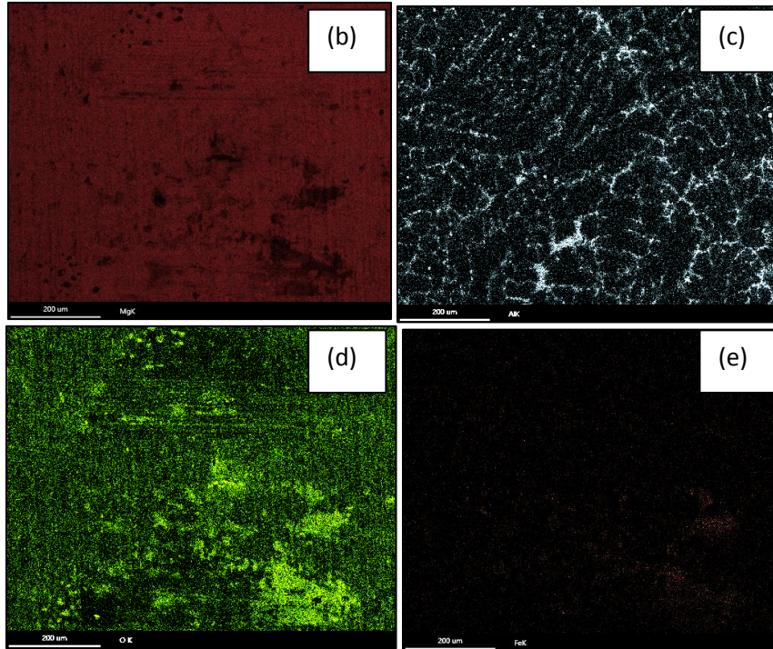
Figure 4.28.(a) SEM micrograph of AM60 alloy worn at 0.2 N 0.1 m/s. EDS maps showing (b) Mg, (c) Al, (d) O and (e) Fe
