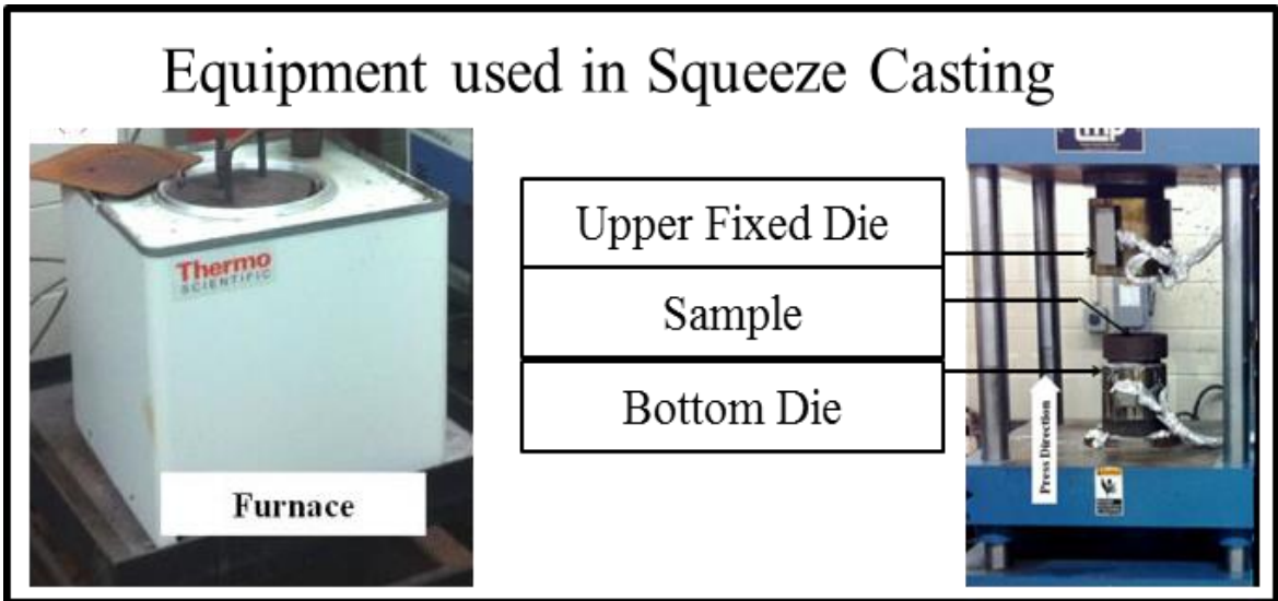
Figure 3.3. Furnace and hydraulic press used for squeezed casting
