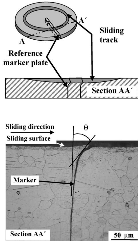
Figure 2.29. (a) Geometry of the marker inserted in the sample (disc) and the cross-section AA`representing the displacement of the marker underneath the contact surface after the sliding wear test and (b) Cross-sectional optical micrograph showing the displacement of the marker towards the sliding direction after sliding for 50 cycles at 673K. [65]
