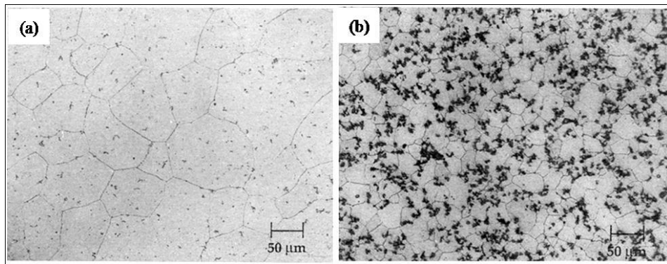
Figure 2.2. Optical micrographs of (a) unreinforced AZ91 alloy and (b) AZ91/SiC composite [23,27].
