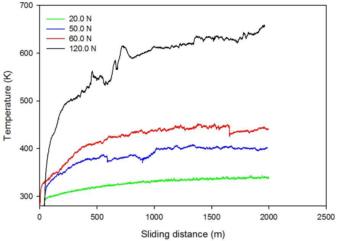
Figure 4.58. Temperature plots for AM60-9% (Al_2O_3)_f composite tested at 1.5 m/s
