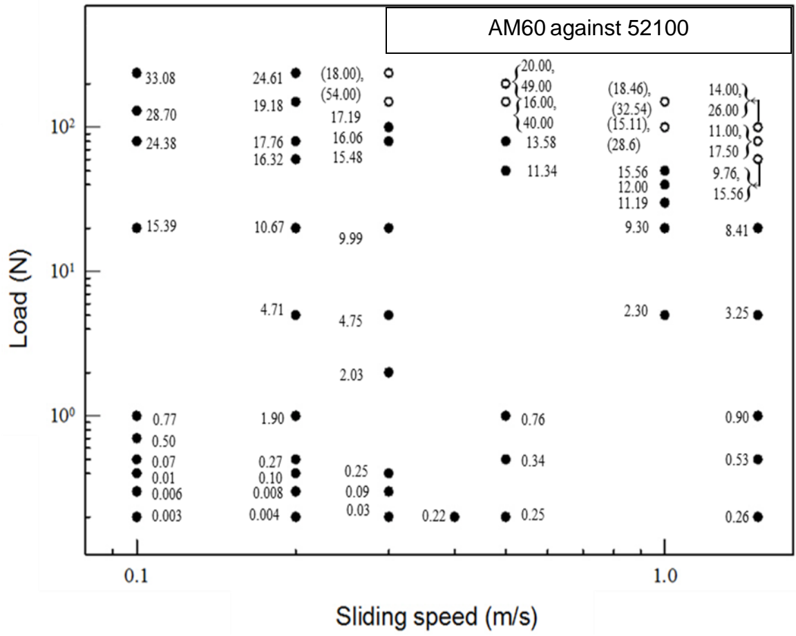
Figure 4.42. Wear rate map for AM60 alloy.
