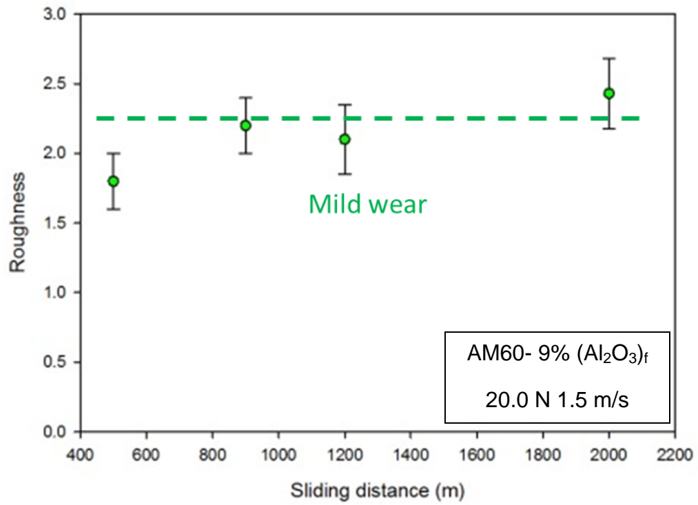
Figure 5.10. Roughness plot for AM60-9% (Al 2 O 3 ) f composite at 20.0 N and 1.5 m/s.
