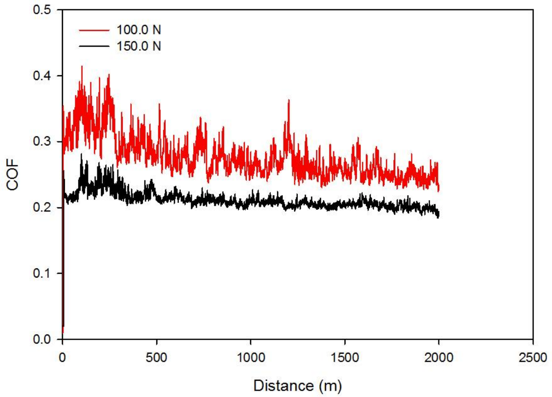
Figure 4.45. COF plots for AM60 alloy tested at 0.3 m/s
