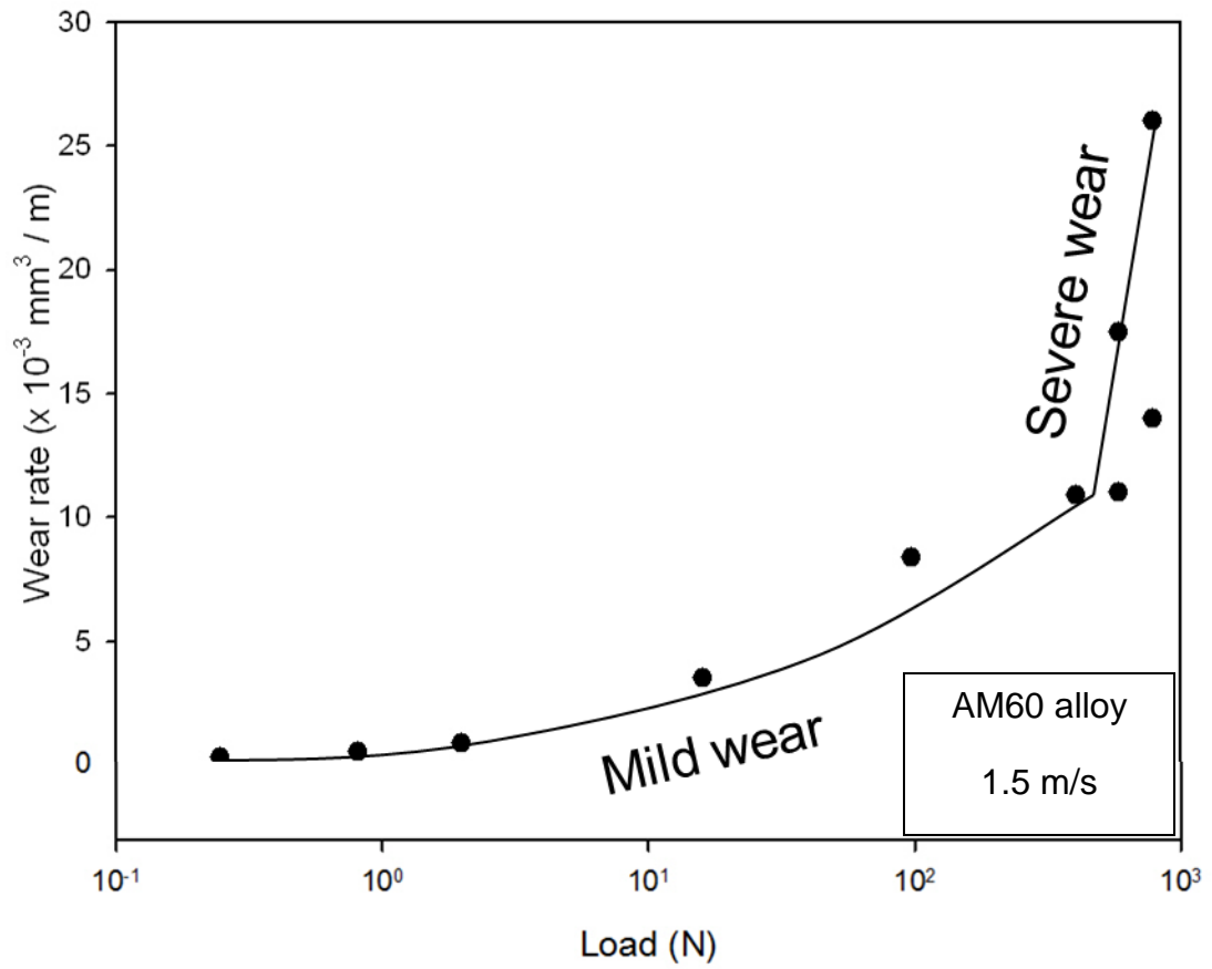
Figure 4.18. Wear rate vs load curve for AM60 alloy at 1.5 m/s.
