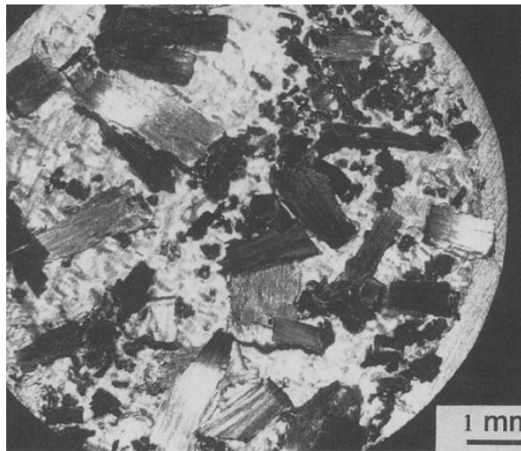
Figure 2.23. Optical micrograph showing (a) Typical morphology of the worn surfaces in the severe wear regime; (b) Wear debris, load = 98 N, v = 0.8\text{m/s} . [57].
