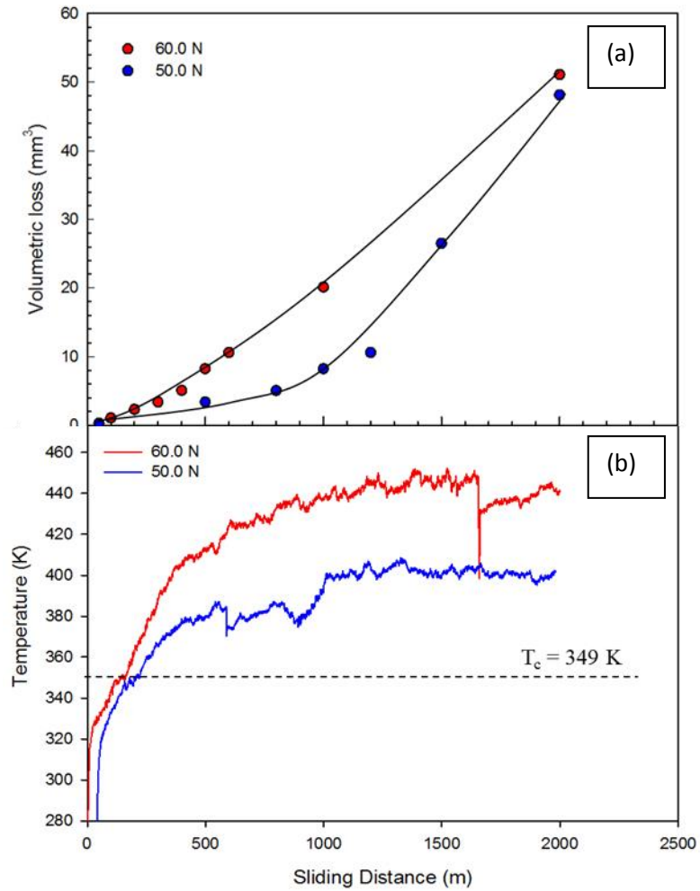
Figure 5.13. (a) Volumetric loss vs. sliding distance plot (b) Temperature plot for AM60-9% (Al 2 O 3 ) f composite at 50.0 N and 60.0 N at 1.5 m/s.
