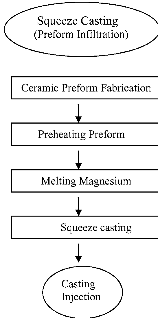
Figure 2.9. Flowchart of squeeze casting process [44].
