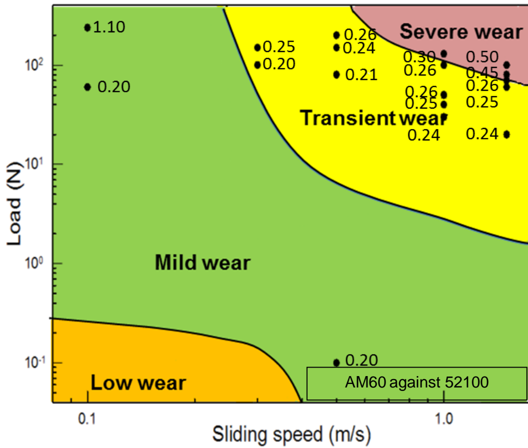
Figure 4.49. COF map for AM60 alloy.
