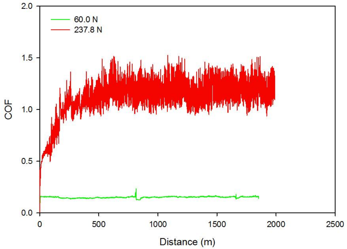
Figure 4.44. COF plots for AM60 alloy tested at 0.1 m/s
