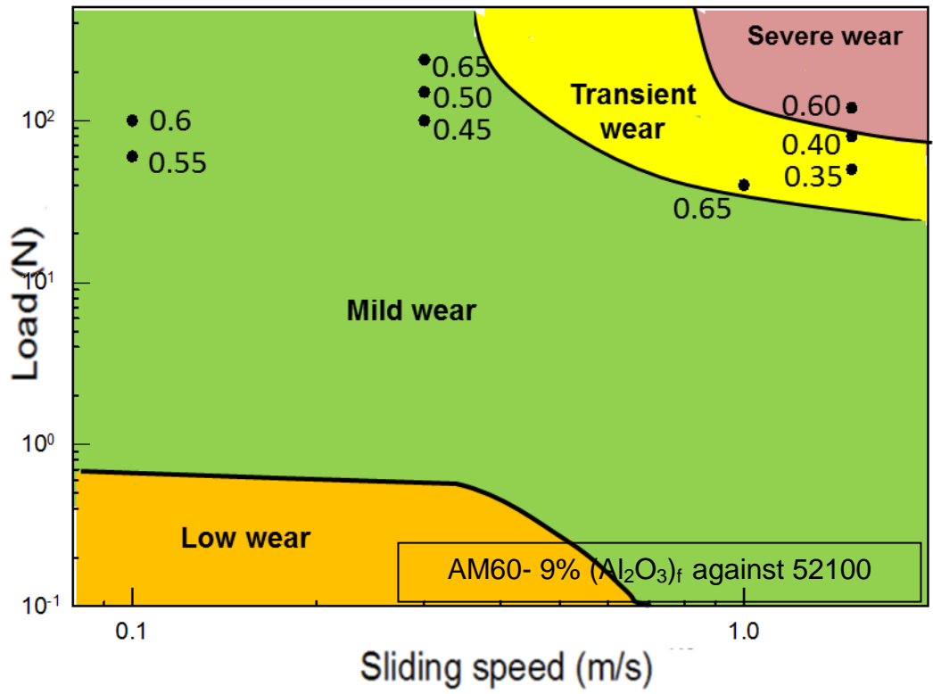
Figure 4.54. COF map for AM60-9% (Al 2 O 3 ) f composite.
