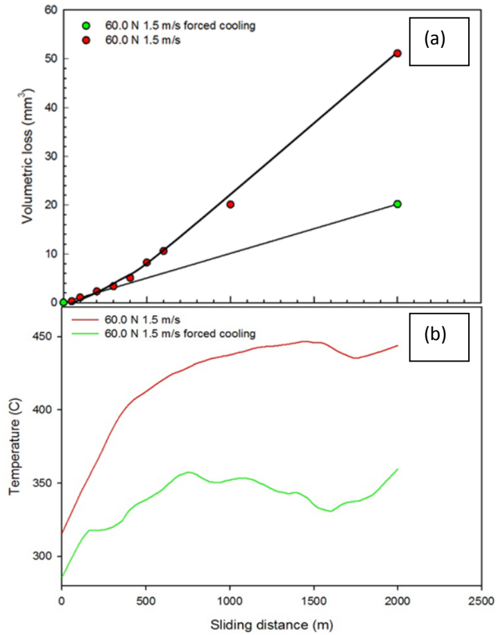
Figure 5.15.(a) Volumetric loss vs. sliding distance plot (b) Temperature plot for AM60-9% (\text{Al}_2\text{O}_3)_f composite at 60.0 N and force-cooled 60.0 N at 1.5 m/s.
