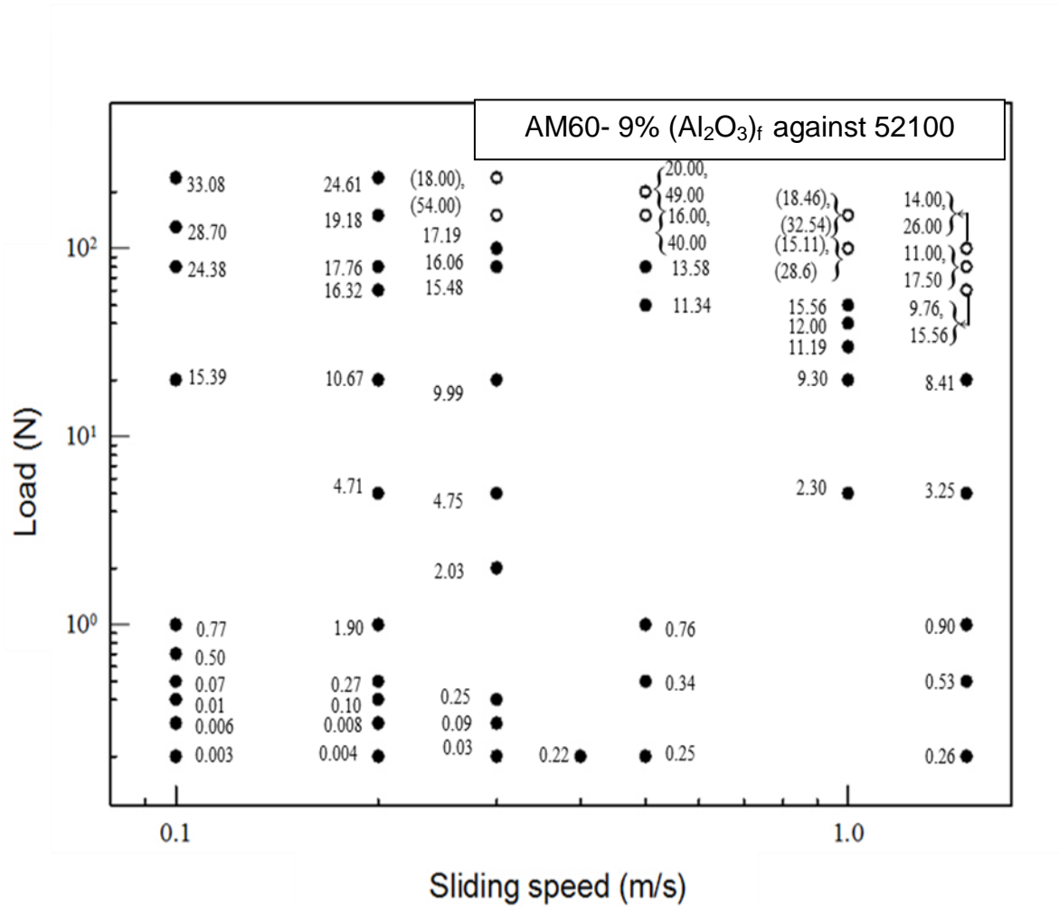
Figure 4.43. Wear rate map for AM60-9% (Al 2 O 3 ) f composite.
