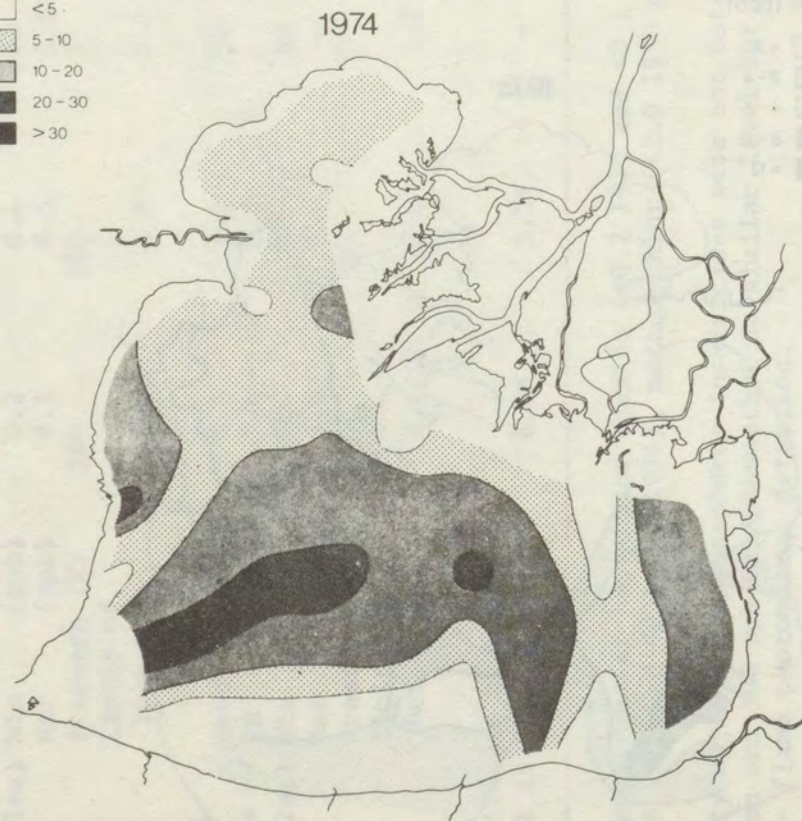
Fig. 2.2-6 Distribution of PCBs in freeze-dried sediments from Lake St. Clair; 1970 and 1974 (0-2 cm).
