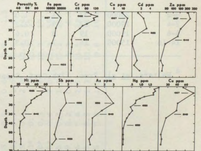
Fig. 1.2-13 Porosity and heavy metal depth profiles for core 4-1 from the western basin of Lake Erie.
