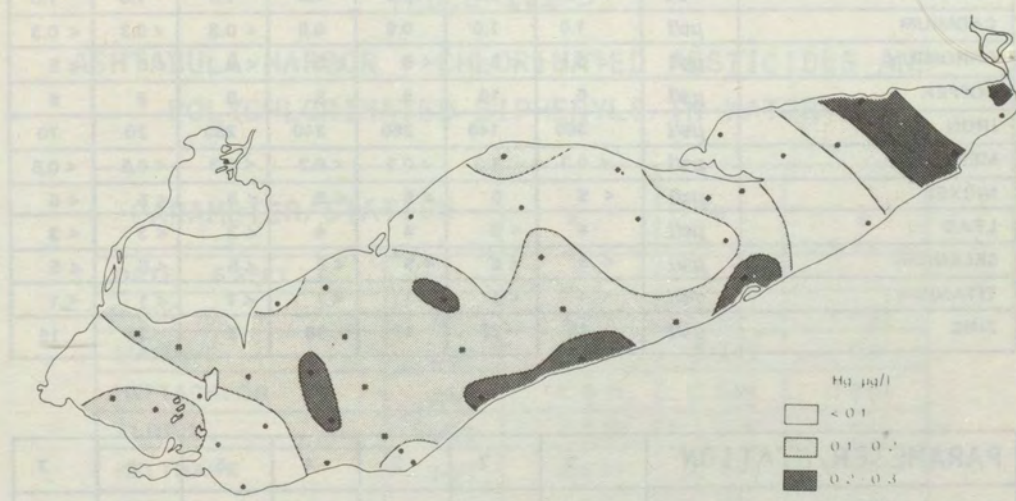
Fig 1.1-2 The average distribution of total mercury in the bottom waters of Lake Erie (1970-1971). Dots represent sampling stations.
