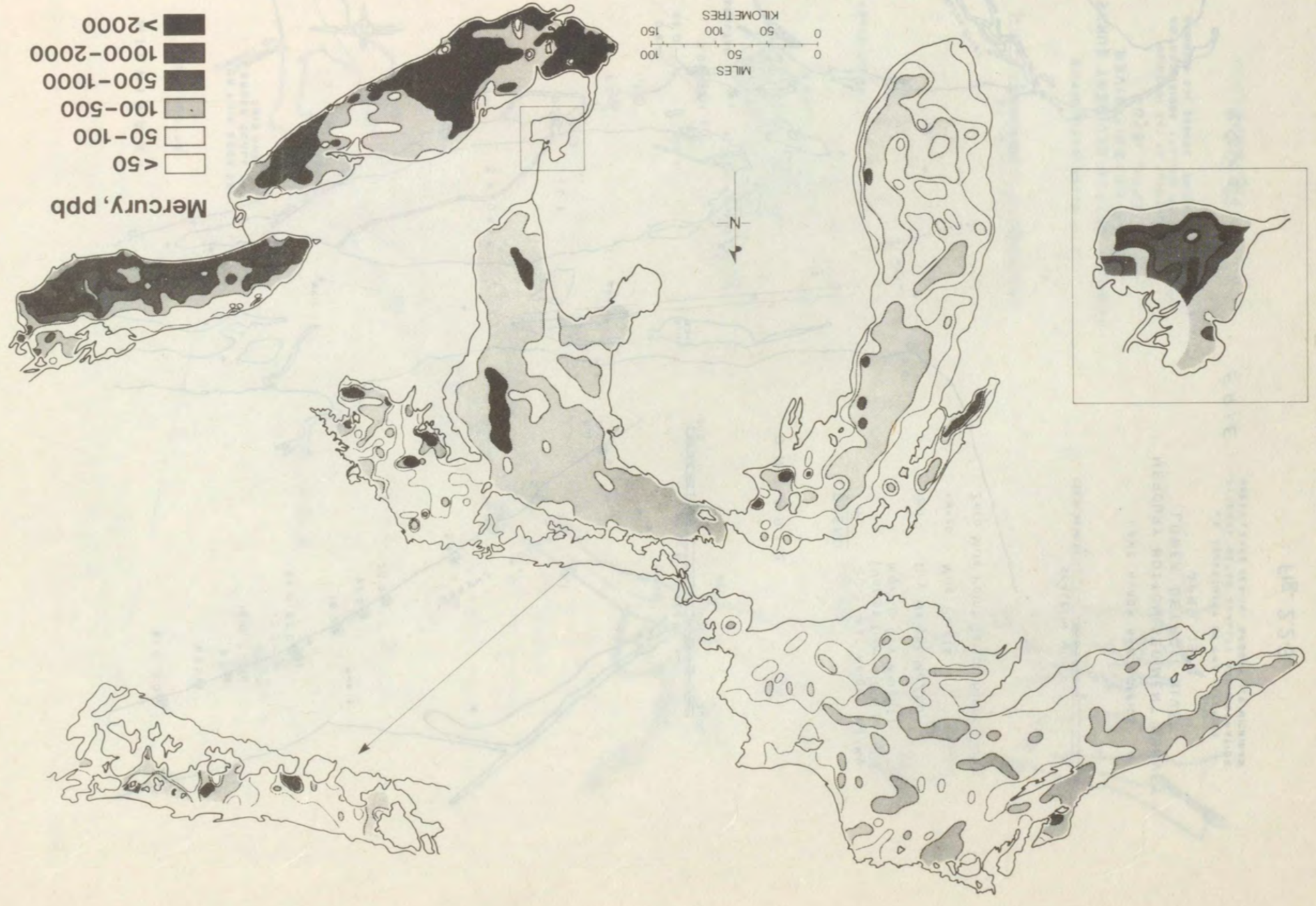
FIGURE 2.2-4. MERCURY CONCENTRATIONS IN SURFACE SEDIMENTS OF THE GREAT LAKES (PPB - JG/KG).
