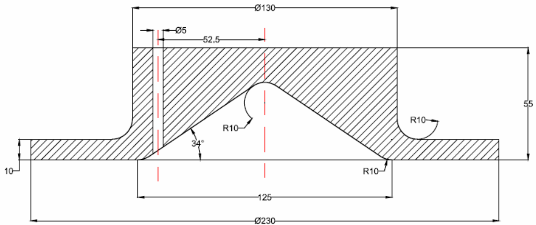
Figure 3.8. Section view of the 34° conical die
