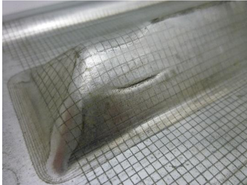
Figure 5.4. Crack in a 1.5 mm DP600 specimen formed into the 38° V-shaped die using a 14 kV pulse
