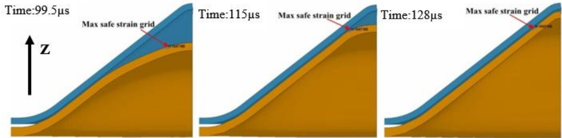
Figure 5.22. Position of the grid that reaches the maximum safe strain at distinct moments during the deformation of the V-shaped specimen
