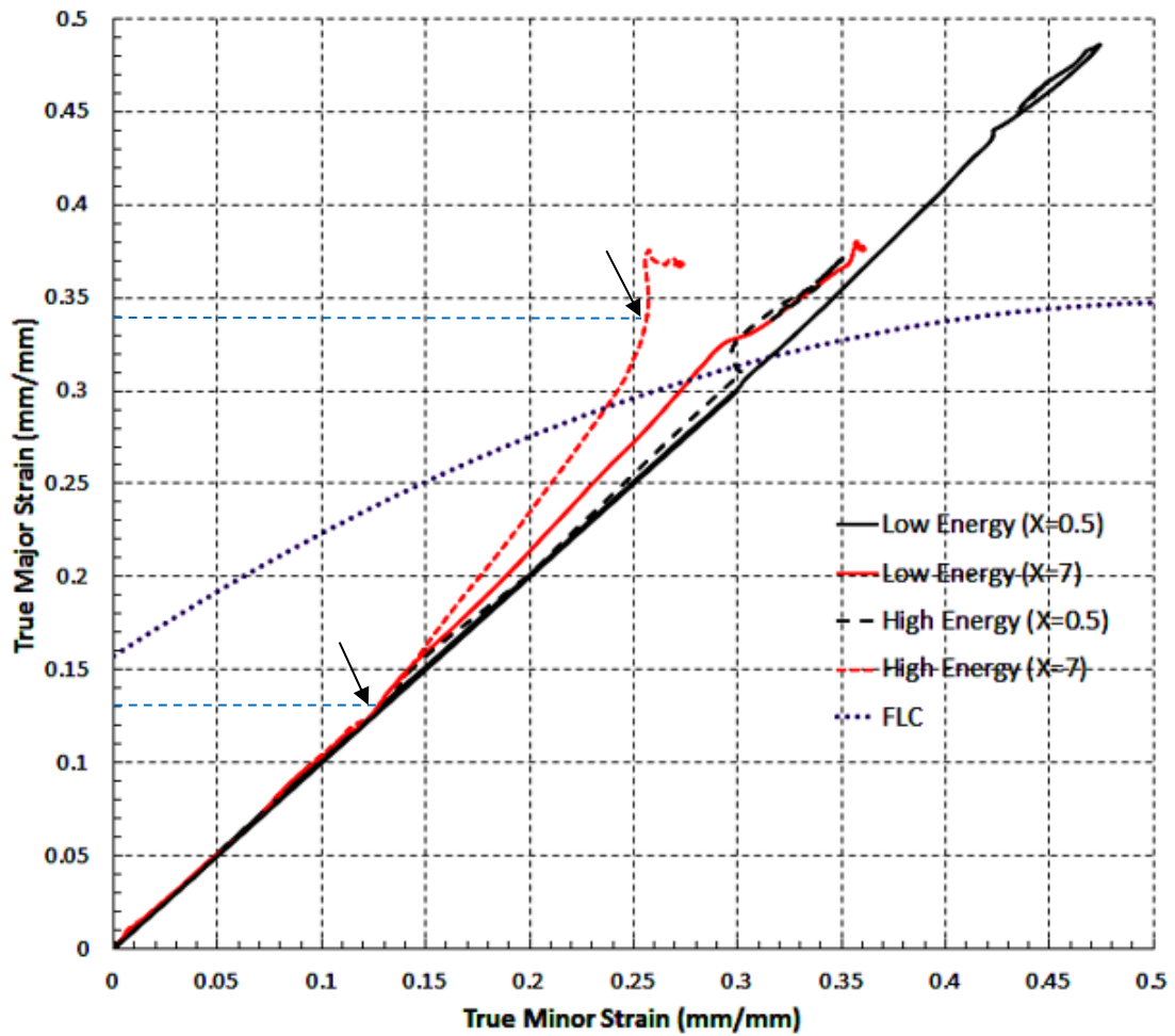
Figure 5.31. The influence of discharge energy on the strain path of selected points
