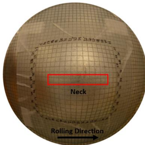
Figure 5.41. EHFF specimen formed in balanced biaxial tension using 13.6kV
