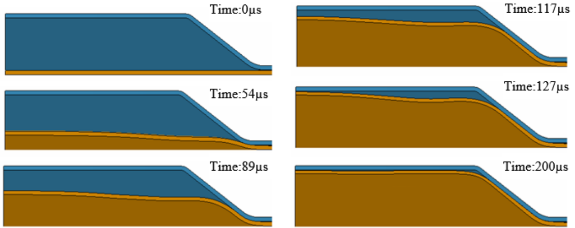
Figure 5.10. Step-by-step sequence of deformation of DP600 sheet during EHDF into the 38° V-shaped die (front view)
