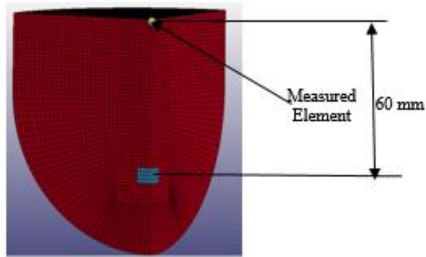
Figure 4.3. Underwater explosion model for element size determination
