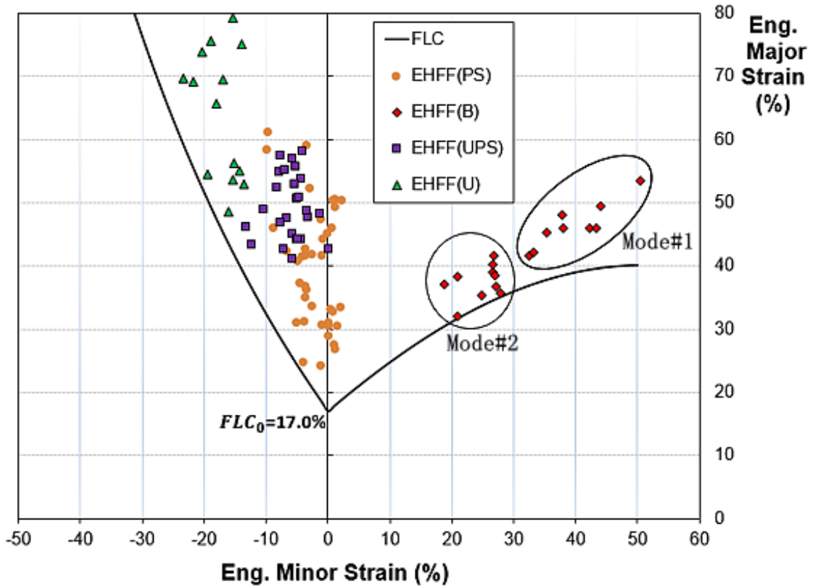
Figure 5.42. Necked strain data measured in different DP600 EHFF specimens (courtesy of Maris, 2014); * deformed in plane strain (PS), biaxial tension (B), uniaxial tension (U) and in and intermediate draw (UPS) mode; strain data in mode #1 come from necked grids right at, or less than 3 grids from, the pole; strain data in mode #2 come from necked grids at least 3 grids away from the pole of the specimen.
