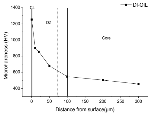
Microhardness gradient-DI-OIL
