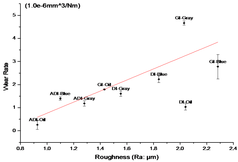
Figure 4.59: Function of wear rate against surface roughness
