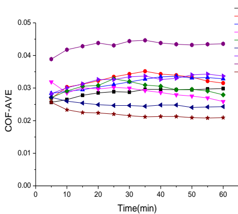
(k) The average of the COF of cast irons
