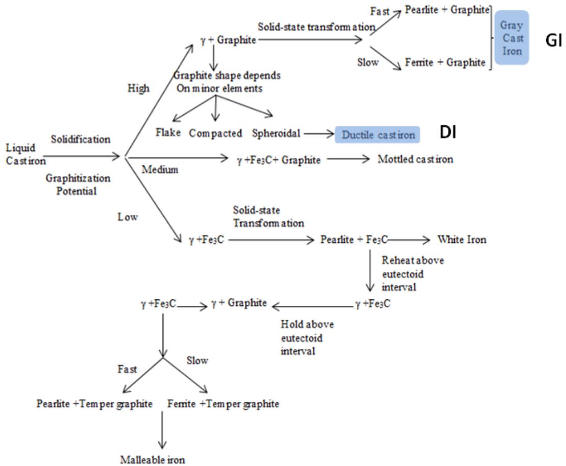
Figure 2.4: Basic microstructures and processing for obtaining common cast irons[1]
