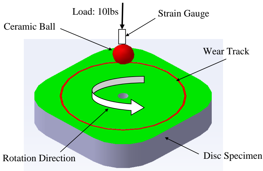
Figure 3.3: Schematic illustration of ball on disc wear test apparatus
