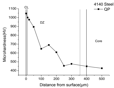
Microhardness gradient-4140 Isonite
