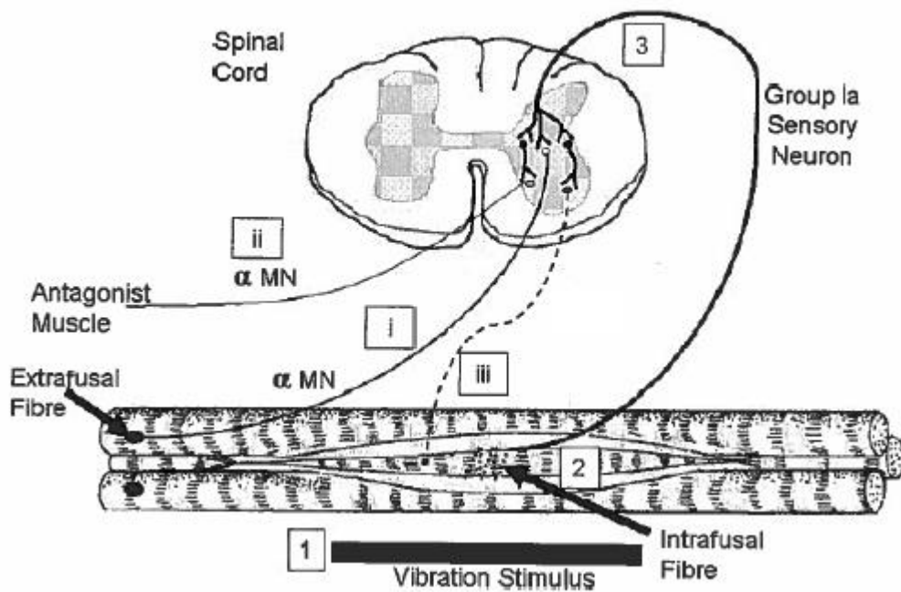
Figure 3: Tonic Vibration Reflex – The vibration stimulus (1) causes changes to muscle length which is detected by the muscle spindles (2) and send Ia sensory neurons to the spinal cord (3). While in the spinal cord, Ia sensory neurons can: (i) mono-synaptically excite \alpha MN to stimulate reflexive muscle contraction of the agonist muscle (extrafusal fibre), (ii) poly-synaptically inhibit \alpha MN to relax antagonist muscle, (iii) poly-synaptically excite intrafusal muscle fibres of agonist muscle to maintain sensitivity to future oscillations. (Hazell, 2006).
