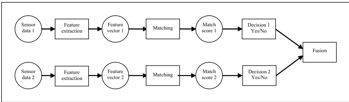
Figure 2.6: Block diagram of fusion at the matching score level
