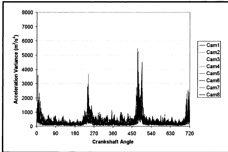
Figure D.2: Comparison of variance for all 8 cams at 1500 RPM.
