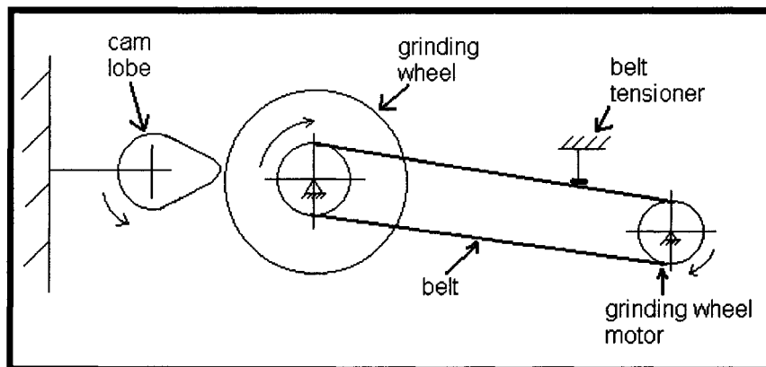
Figure 4.2: Schematic of camshaft machining process.
