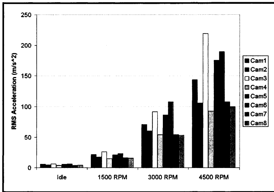
Figure 6.1: 30-cycle RMS acceleration for each camshaft at different engine speeds.
