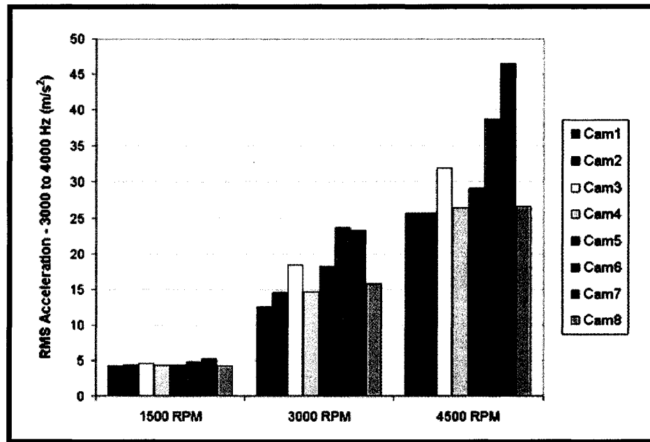
Figure 6.7: Band-limited RMS vibration for the eight camshafts.
