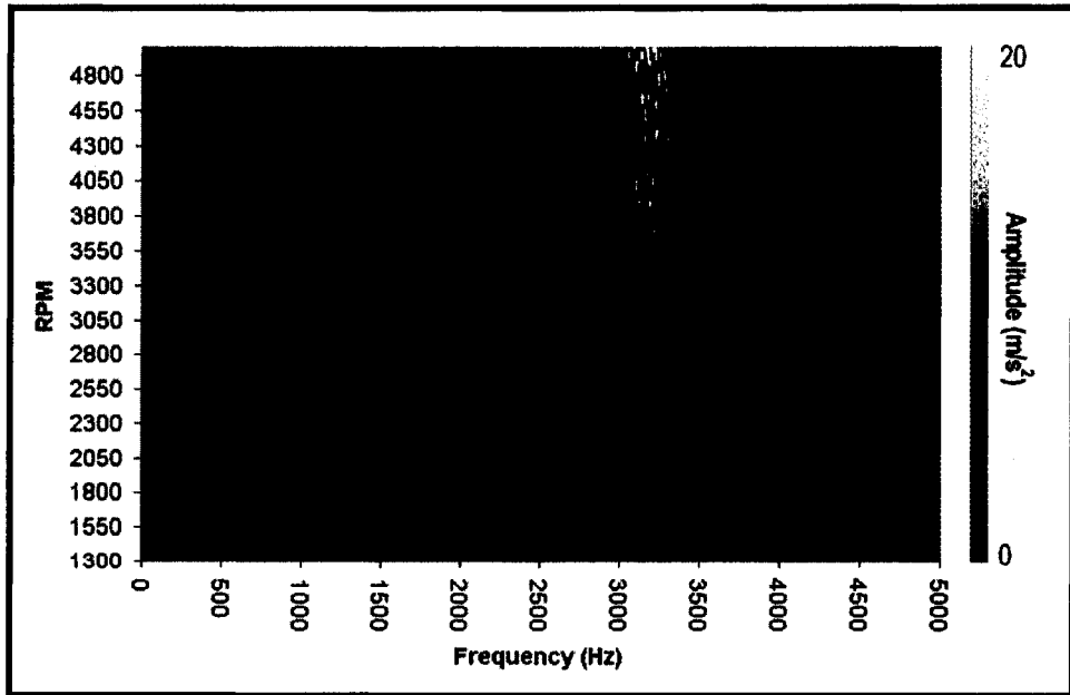
Figure E.4: Color map for camshaft #4.
