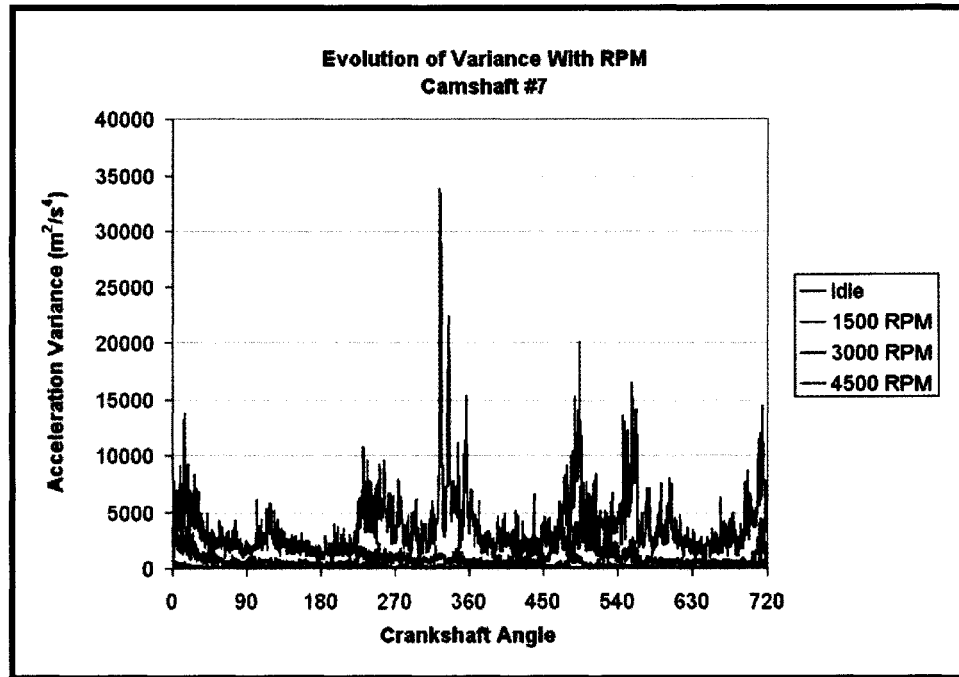
Figure C.7: Evolution of variance with RPM for camshaft #7.
