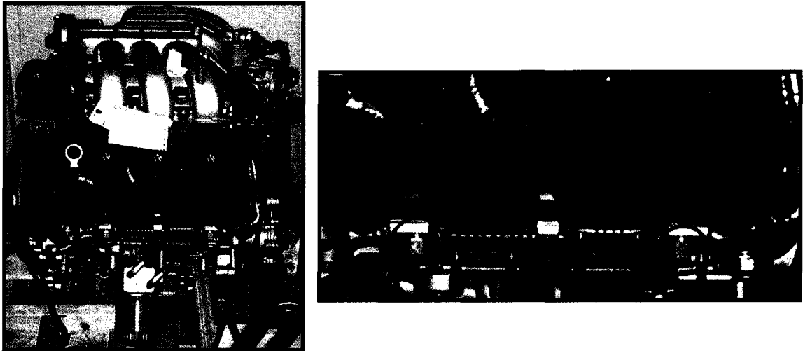
Figure 4.3: Full view (left) and close-up of V6 showing accelerometer locations (red circles).
