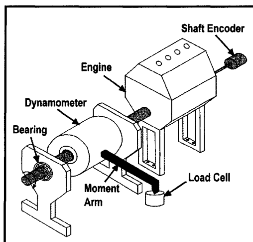
Figure 3.10: Schematic of a typical engine dynamometer setup.
