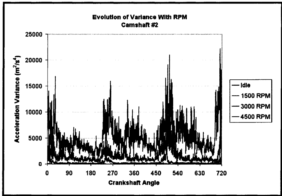
Figure C.2: Evolution of variance with RPM for camshaft #2.
