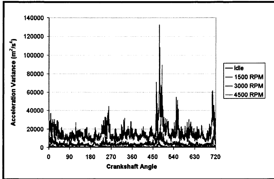
Figure 6.3: Evolution of variance with engine RPM.
