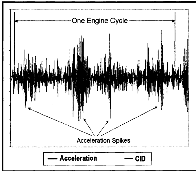
Figure B.3: Acceleration signal acquired from vicinity of defective cylinder.
