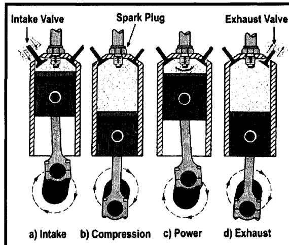
Figure 3.1: The S.I. Engine 4-stroke cycle.
