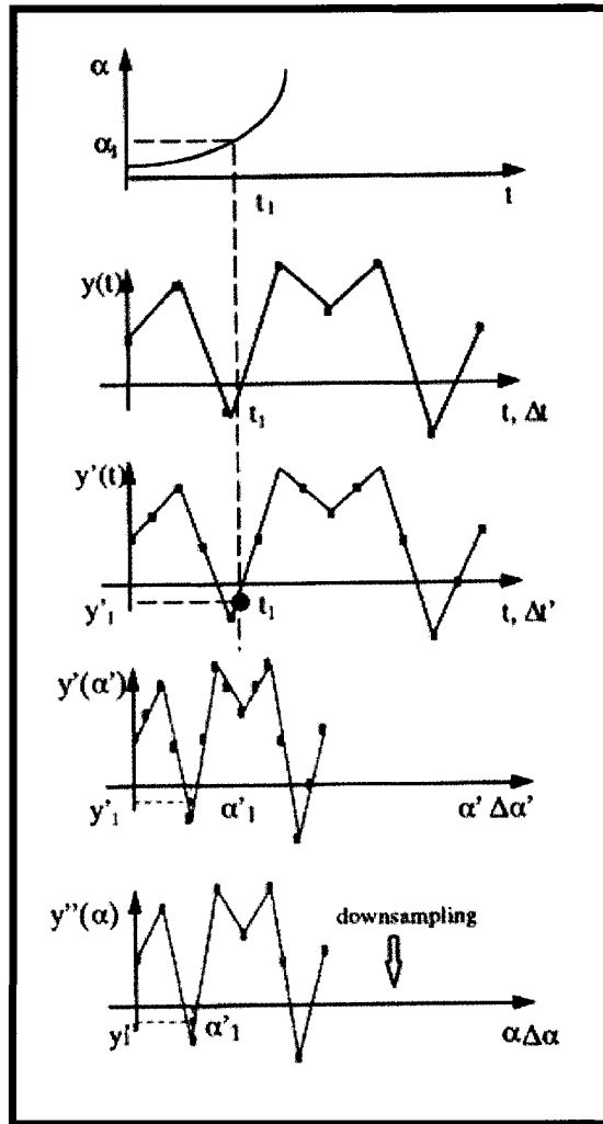
Figure 3.22: Synchronous re-sampling.
