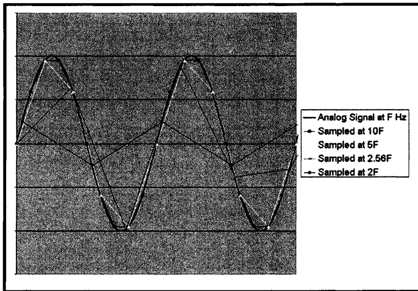
Figure 3.12: Reproduction of sine wave with different sampling rates.
