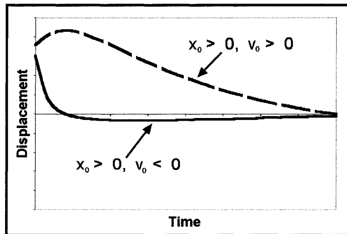
Figure 3.8: Examples of critically damped motion ( \zeta=1 ).
