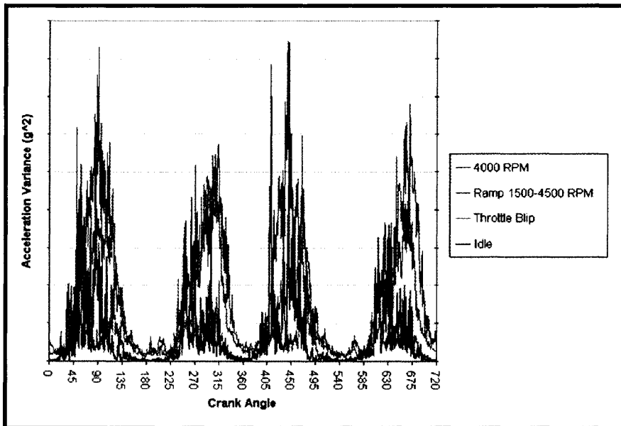
Figure B.4: Variance plots for each of the investigated conditions.
