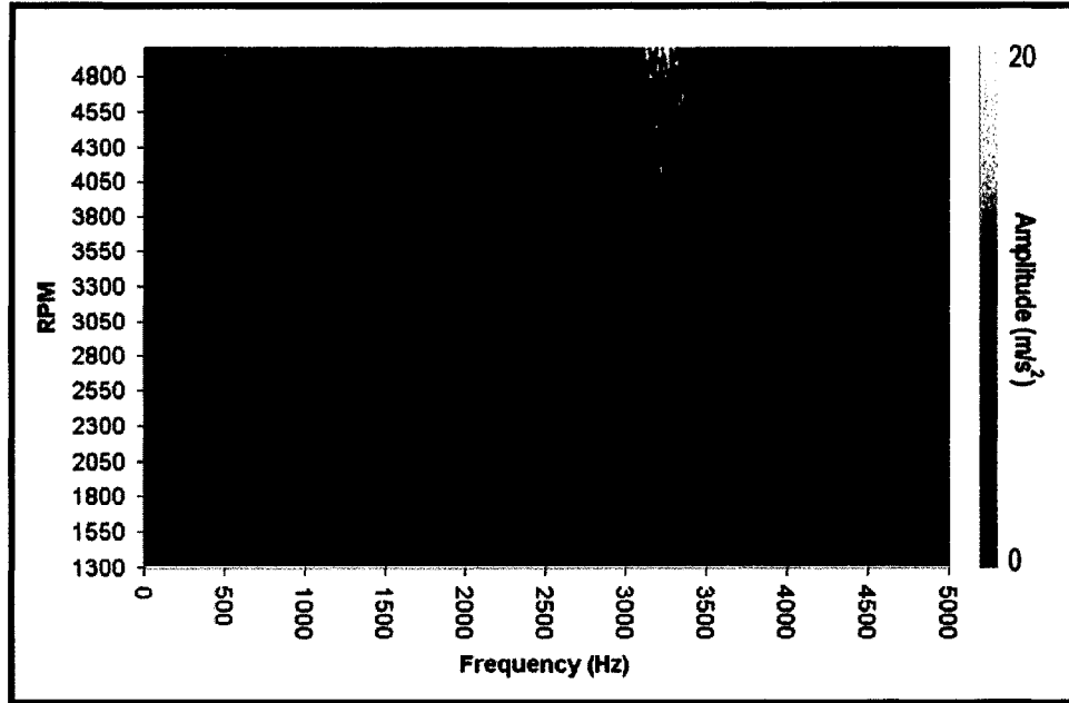
Figure E.3: Color map for camshaft #3.
