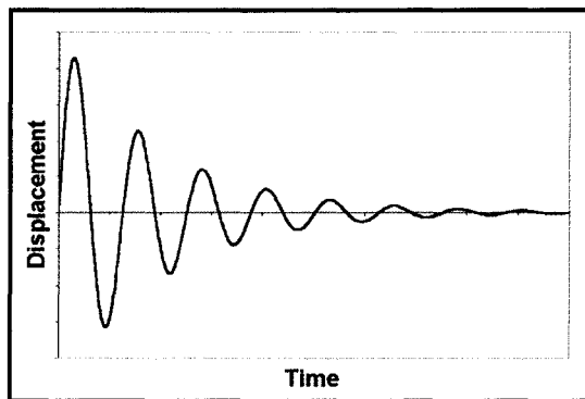
Figure 3.7: Example of underdamped response ( \zeta < 1 ).
